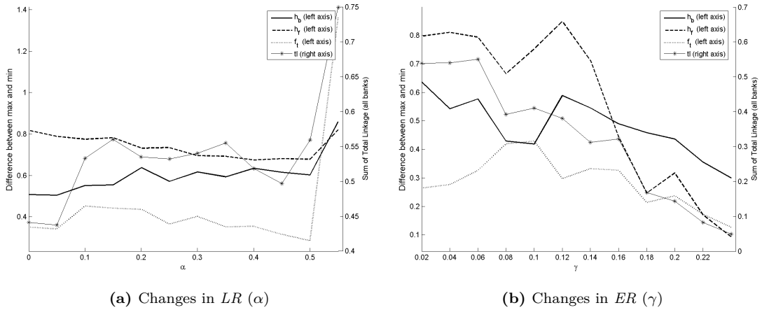
Figure 14: IO measures: max - min ( \bar{h}_b , \bar{h}_f , \bar{f}_t , left axis) and sum over all banks ( tl , right axis)
