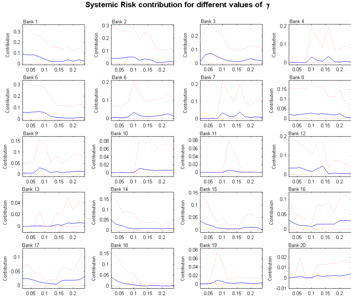
Figure 16: Contribution to systemic risk (Shapley Value) by bank for different values of \gamma and for the RAS network
