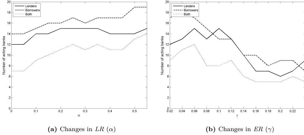
Figure 13: Number of active banks in interbank market for different values of \alpha and \gamma
