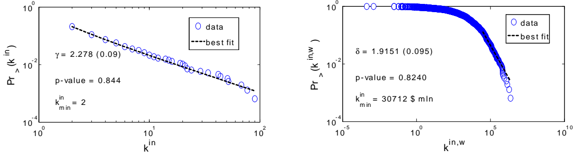
Figure 3: The cumulative distribution functions and their maximum likelihood power-law fits for: (a) k^{in} and (b) k^{in,w}
