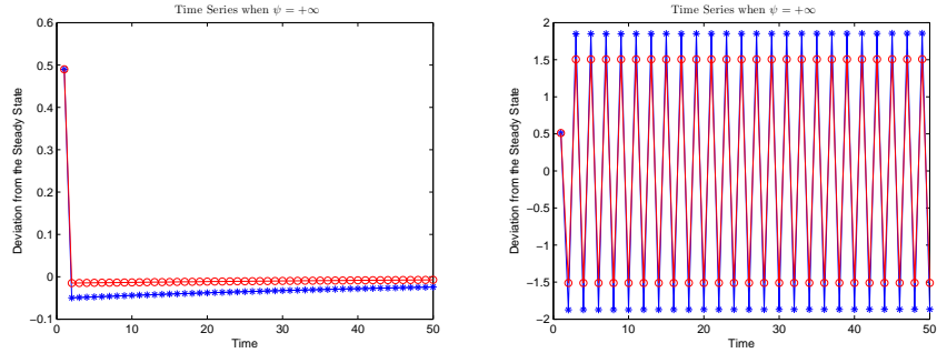
Figure 6: Inflation (red) and output (blue) time series for the case \psi = \infty confirming the results presented in the two above phase plots.
