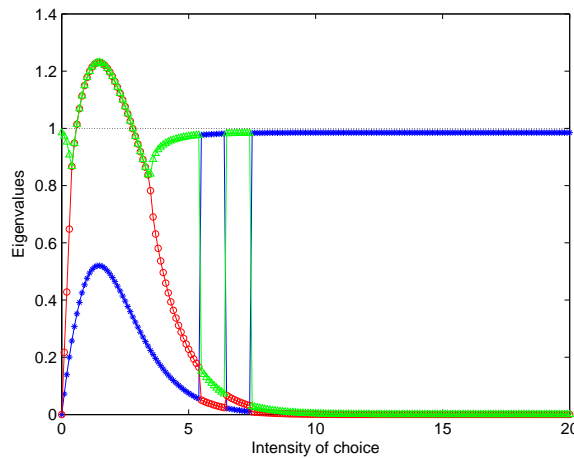
Figure 3: A representation of the three eigenvalues ( \lambda_1 in blue, \lambda_2 in red and \lambda_3 in green) as a function of the intensity of choice parameter.
