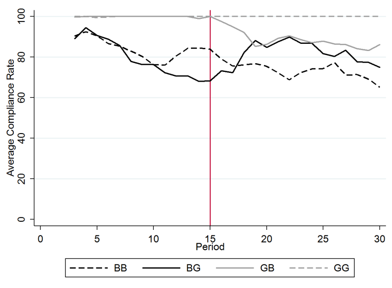
Figure C.3: Inequity-averse players
