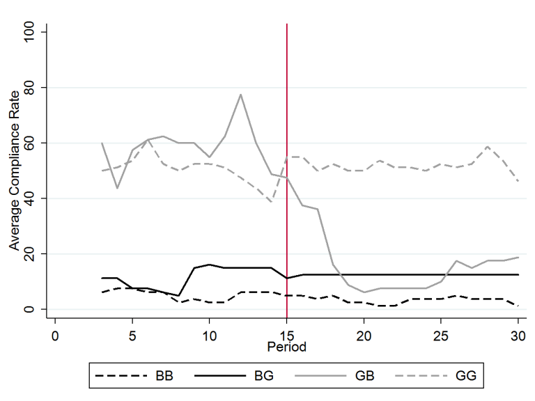
Figure C.2: Selfish players
