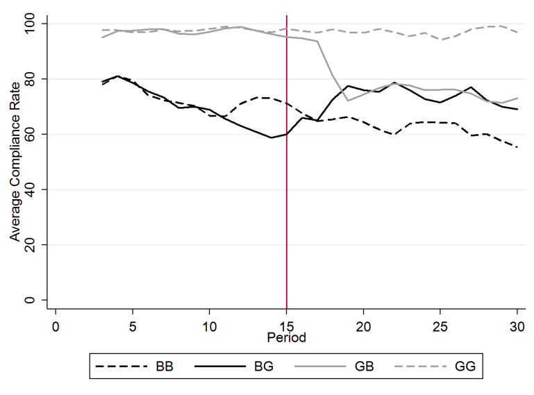
Figure C.4: Evasion-averse players
