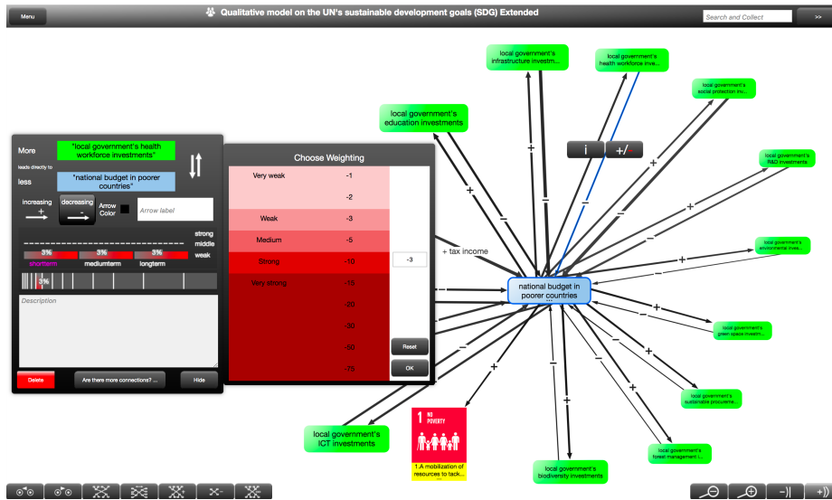
Fig. 4. An example the qualitative weighting of connections.
