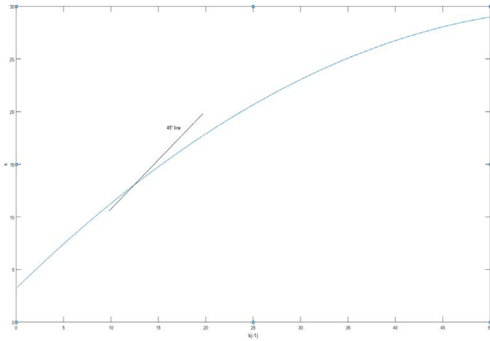
Figure 2: Policy function for k_t
