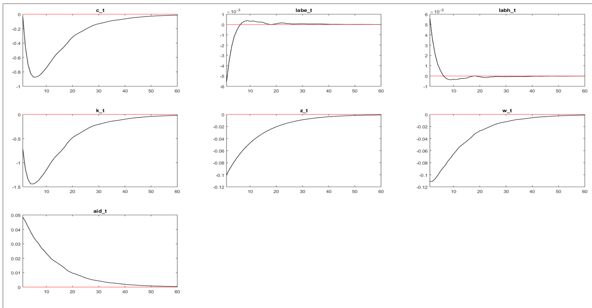
Figure 3. Impulse response functions of a one standard deviation shock of \varepsilon
