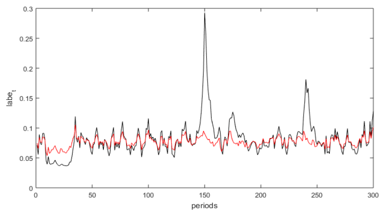
Figure 4. Simulations of the economy with low ( \sigma = 0.1 , red line) and high volatility ( \sigma = 0.2 , black line) Source: Authors' own calculations using Dynare.
