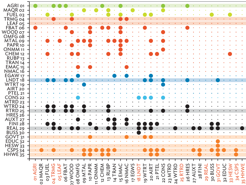
Figure 4: Agglomeration of Economic Sector-Specific Productive Activities Using the Dot-Plot Matrix Representation
