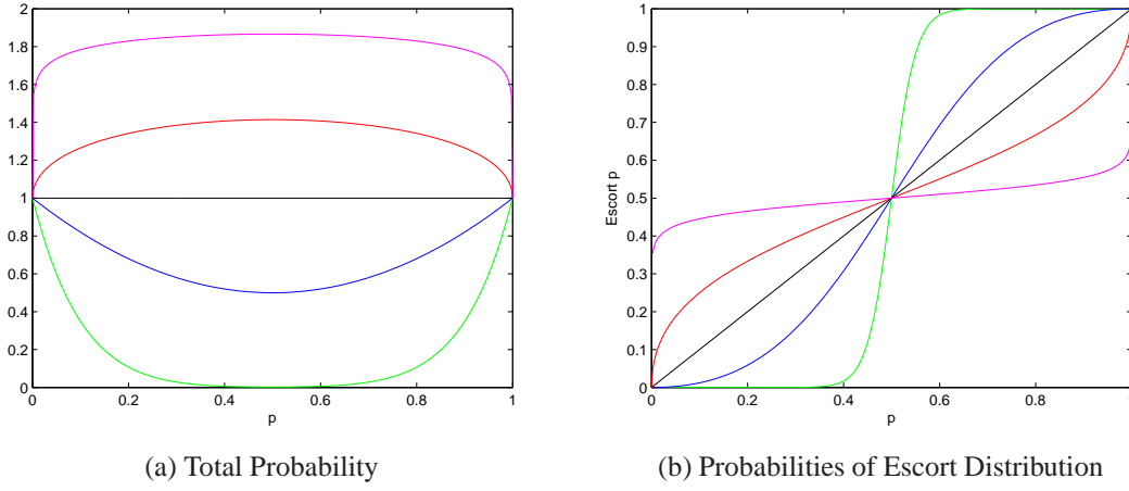
Figure 2: Biased Probabilities
