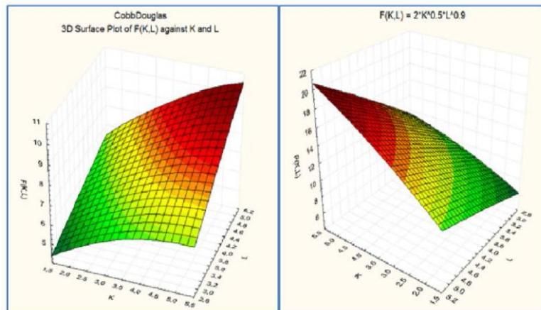
Figure no. 5: Point of view and perspective control for a Cobb-Douglas production function Source: Run with Statistica software
