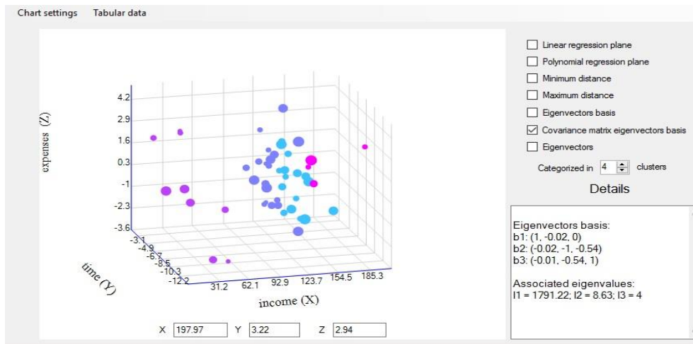
Figure no. 3: Using eigenvectors for data variance analysis
