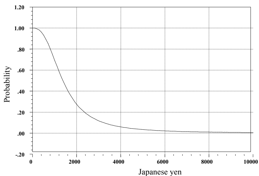
Figure 2. Probability of acceptance (demand function)
