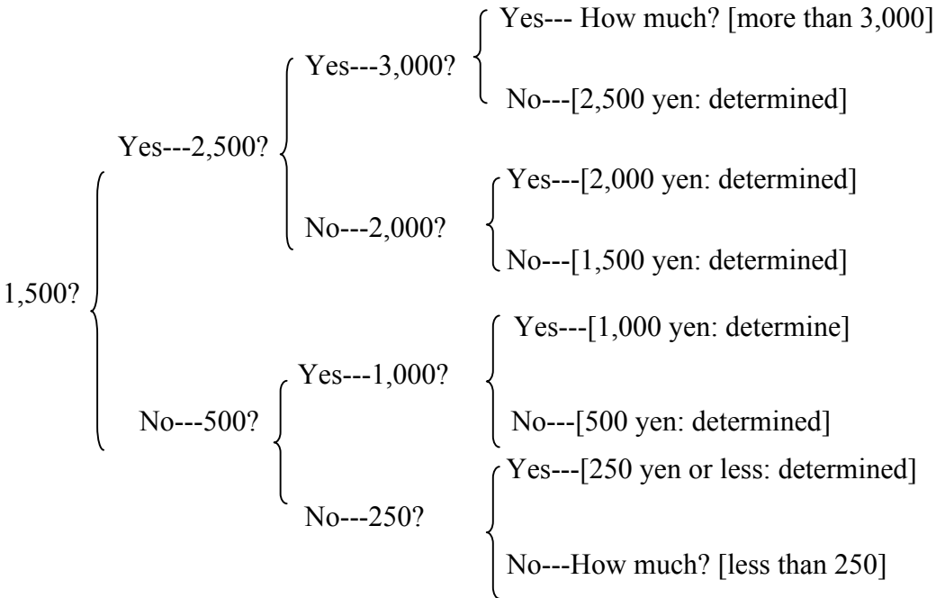
Figure 1. Tree structure of questions
