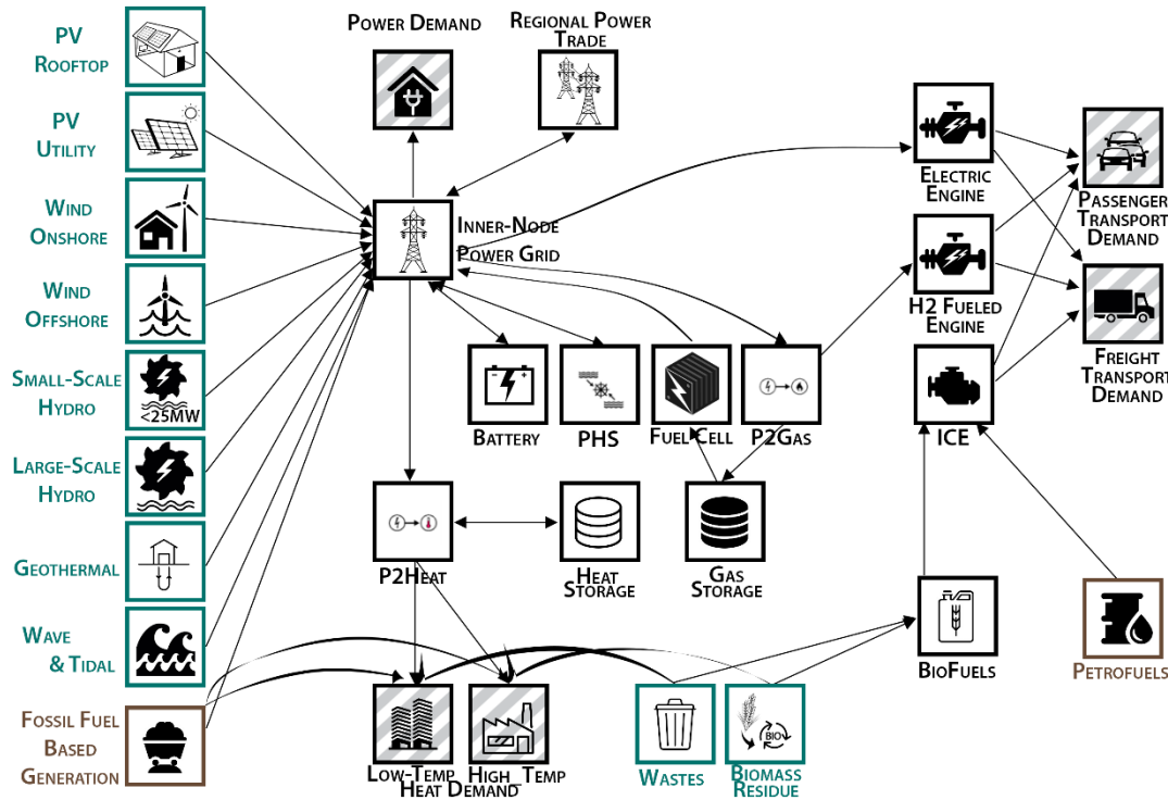
Figure 2: Layout of GENeSYS-MOD
