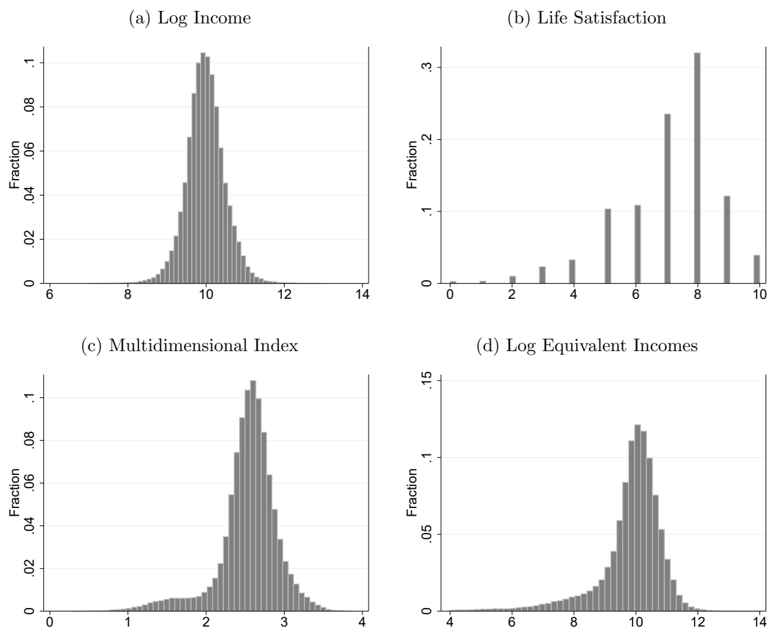
Figure 1: Histograms
