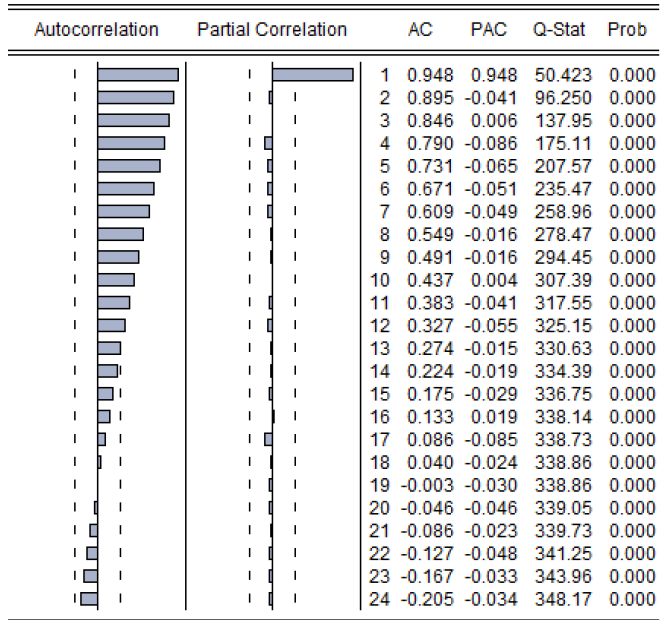
Figure 2: ACF and PACF of lrgdp
