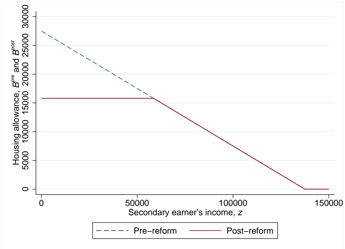
Figure 1: Housing allowance before and after the reform according to the functions B^{pre}(\tilde{z}^p + \tilde{z}) and B^{post}(\tilde{z}^p, \tilde{z}) as a function of secondary income \tilde{z} for a family with two children. The primary earner's income is fixed at \tilde{z}^p = 170,000 .
