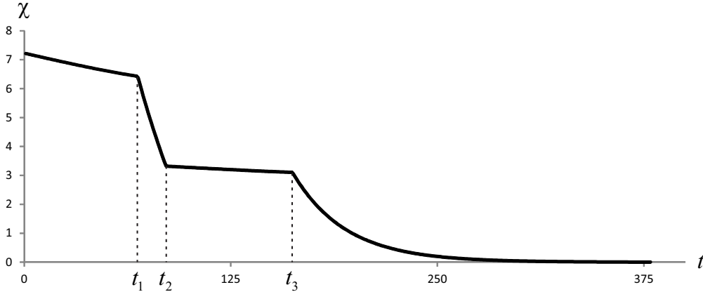
Figure 2: Fossil fuel extraction path for g_0 = 1000 , r = 0.05 , b = 0.9 , q_1 = 0.22 , q_2 = \sigma_1 = \sigma_2 = 0.005 , a_1 = a_2 = 4 , c_1 = c_2 = 1 , \theta = 0.01 , \eta = 0.001
