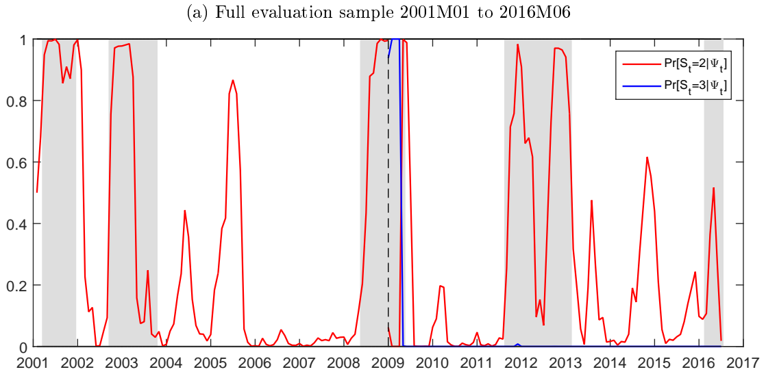
Figure 8: Real-time nowcast of recession probabilities using a MS(2)/MS(3)-DFM
