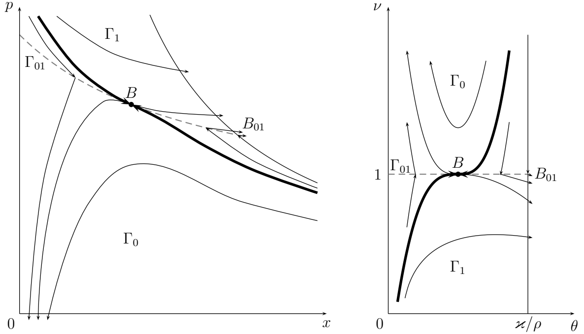
Figure 3: Trajectories of the Hamiltonian system of the PMP for problem (\widehat{P}_1^V) in \Gamma for (1 - \kappa)\delta > \rho (case (c)) in the coordinates (x, p) (left) and (\theta, \nu) (right). In \widehat{\Gamma}_0 these trajectories coincide with those for problem (\widehat{P}_1) . Optimal trajectories are shown by thick lines, and \Gamma_{01} is shown by dashed lines
