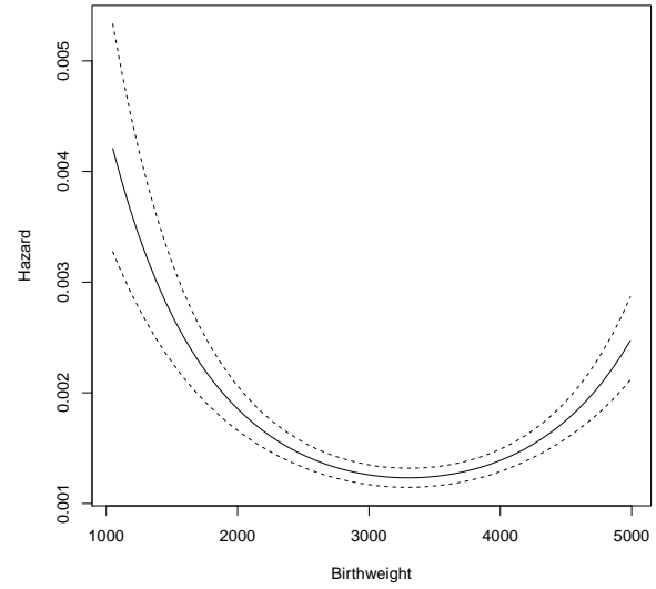
Figure 6: Estimated parametric covariate hazard function.
