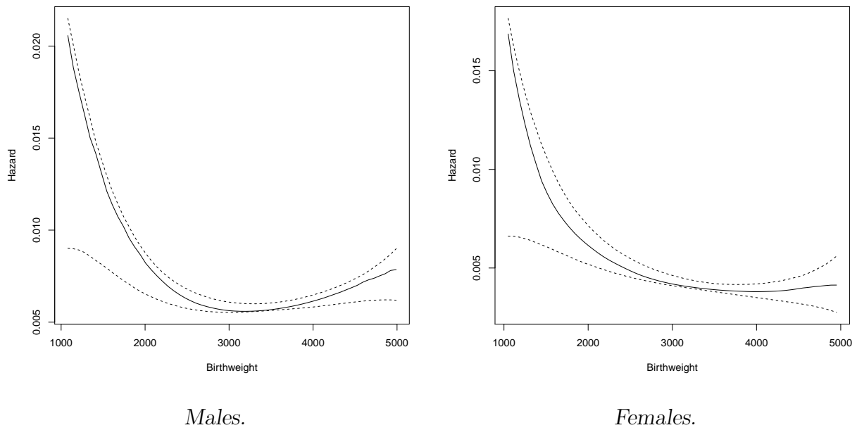
Figure 9: Semiparametric estimation results for g using the local linear estimator, controlling for social class at birth and stratified by gender.
