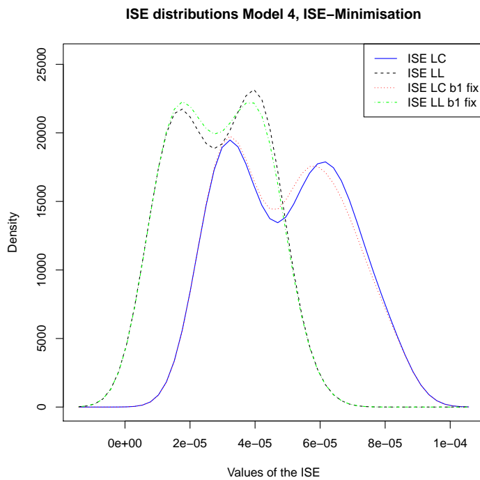
Figure 3: The empirical distributions for the ISE with an optimally chosen b_1 (solid line and dashed line) and with a fixed b_1 (the dotted line and the dot-dash line, for the local constant and the local linear estimator, respectively).
