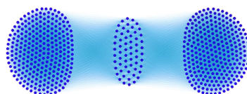
Figure 6. A network with two overlapping cliques, N = 600 and N_{ov} = 60 .
