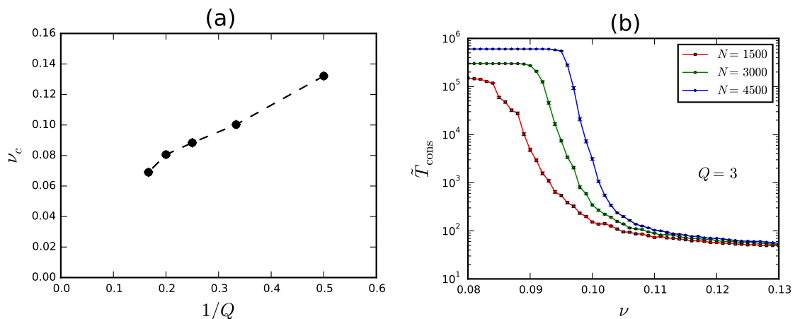
Figure 10. (a) Dependence of \nu_c upon the number Q of communities; (b) Bounded time to consensus from simulations in the PPM with Q = 3 .
