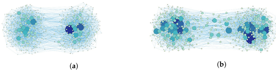
Figure 12. (a) BA communities interconnected by scale-free links (no inter-community assortativity); (b) BA communities interconnected by scale-free links (with inter-community assortativity). In both cases, N = 600 , \rho = 0.1 , the size of each node is proportional to its overall degree and the spatial position of nodes represents the equilibrium configuration of the Force Atlas visualization algorithm [51].
