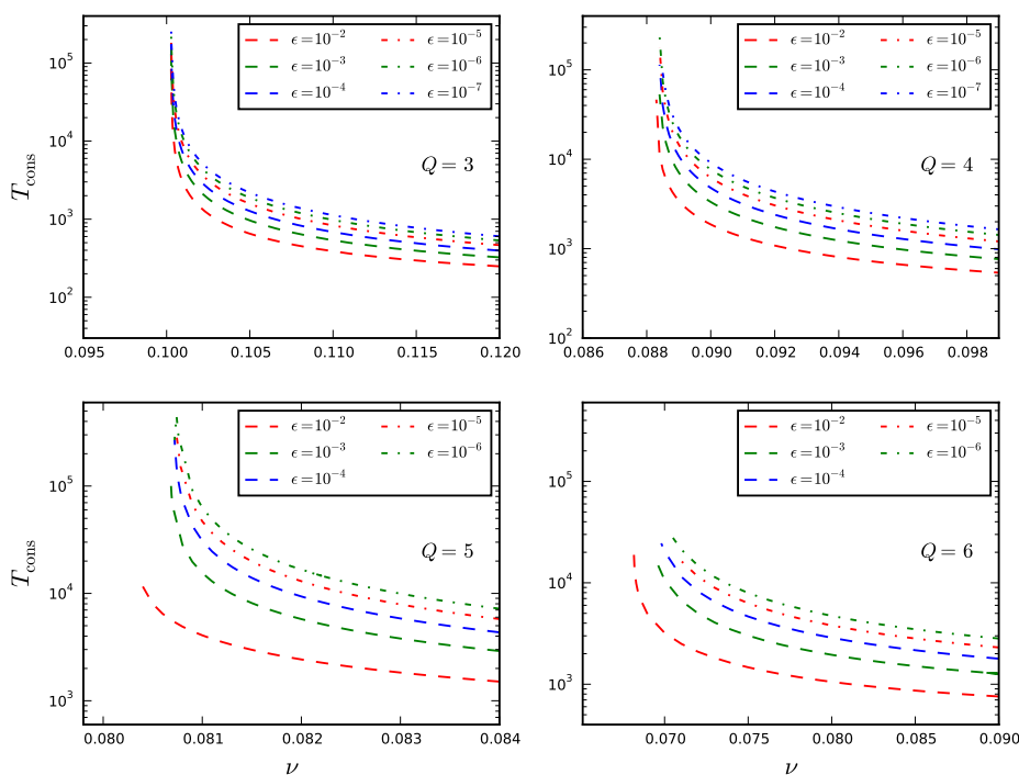
Figure 9. Time to consensus in the PPM with Q > 2 .
