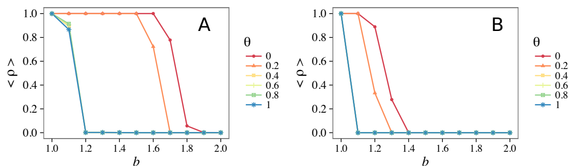
Figure 3. Mixed update rule with q = 0.3 . ER monoplex network. (A) z = 4 ; (B) z = 16 . Average final fractions of cooperators \rho as a function of b for different values of \theta .
