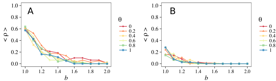
Figure 5. Mixed update rule with q = 0.3 . BA monoplex network. (A) z = 4 ; (B) z = 16 . Average final fractions of cooperators \rho as a function of b for different values of \theta .
