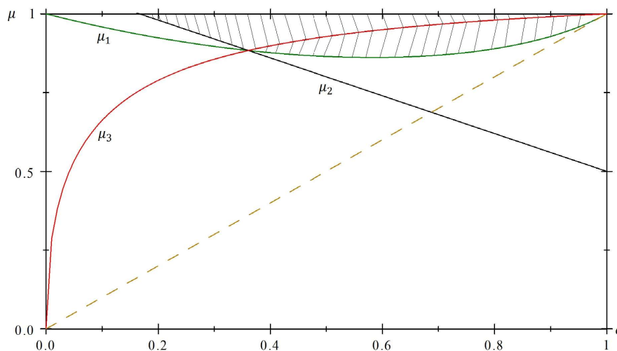
Figure 1. Pairs (\delta, \mu) yielding multiple SPE expected outcomes when n = 11 and n_B = 5 .
