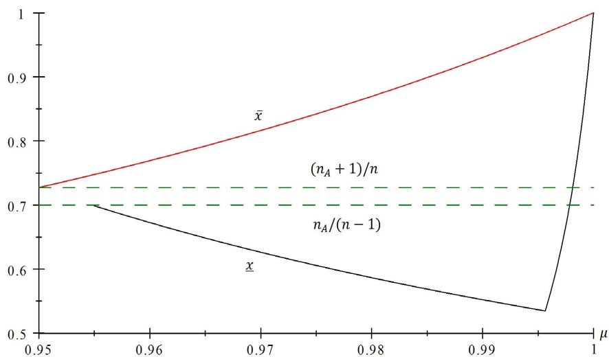
Figure 2. Set of no-delay SPE expected outcomes when n = 11 , n_B = 3 and \delta = 0.95 .
