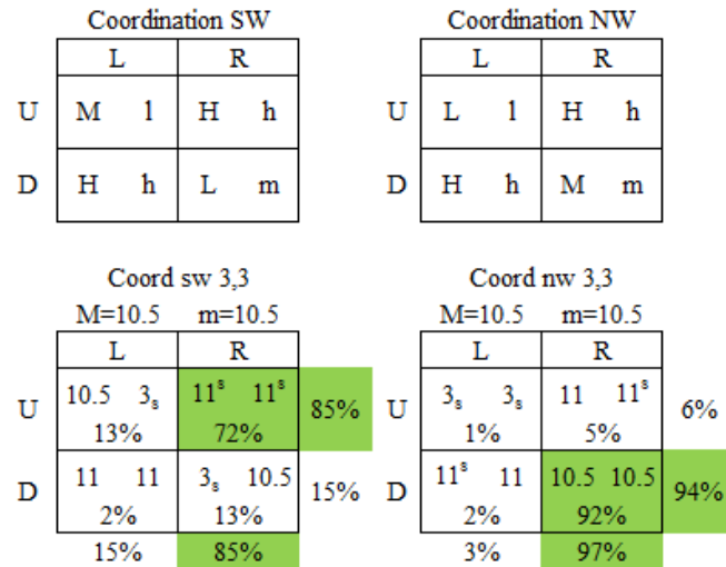
Figure 15. Equilibrium and Disequilibrium Play in Coordination Games.
