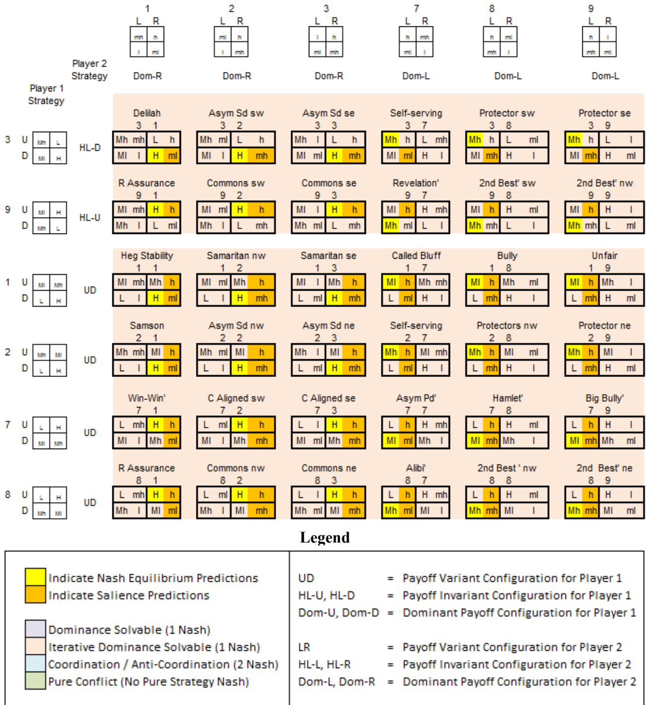
Figure 8. Strictly ordinal 2 \times 2 dominance solvable games with dominant strategy for P2.
