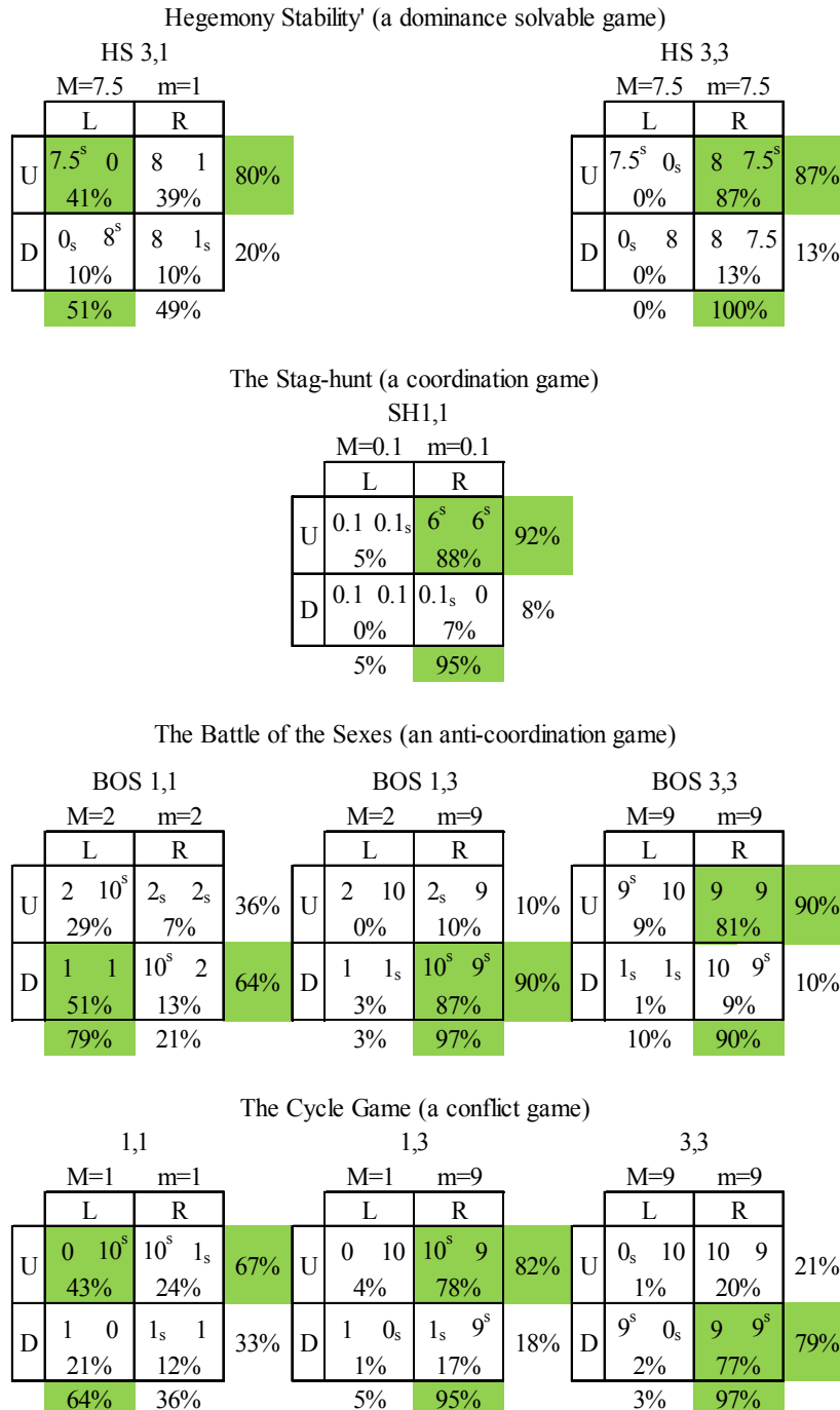
Figure 16. Payoff Variant Games.
