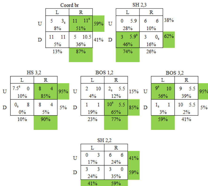
Figure 18. “Other Payoff” Solvable Games.
