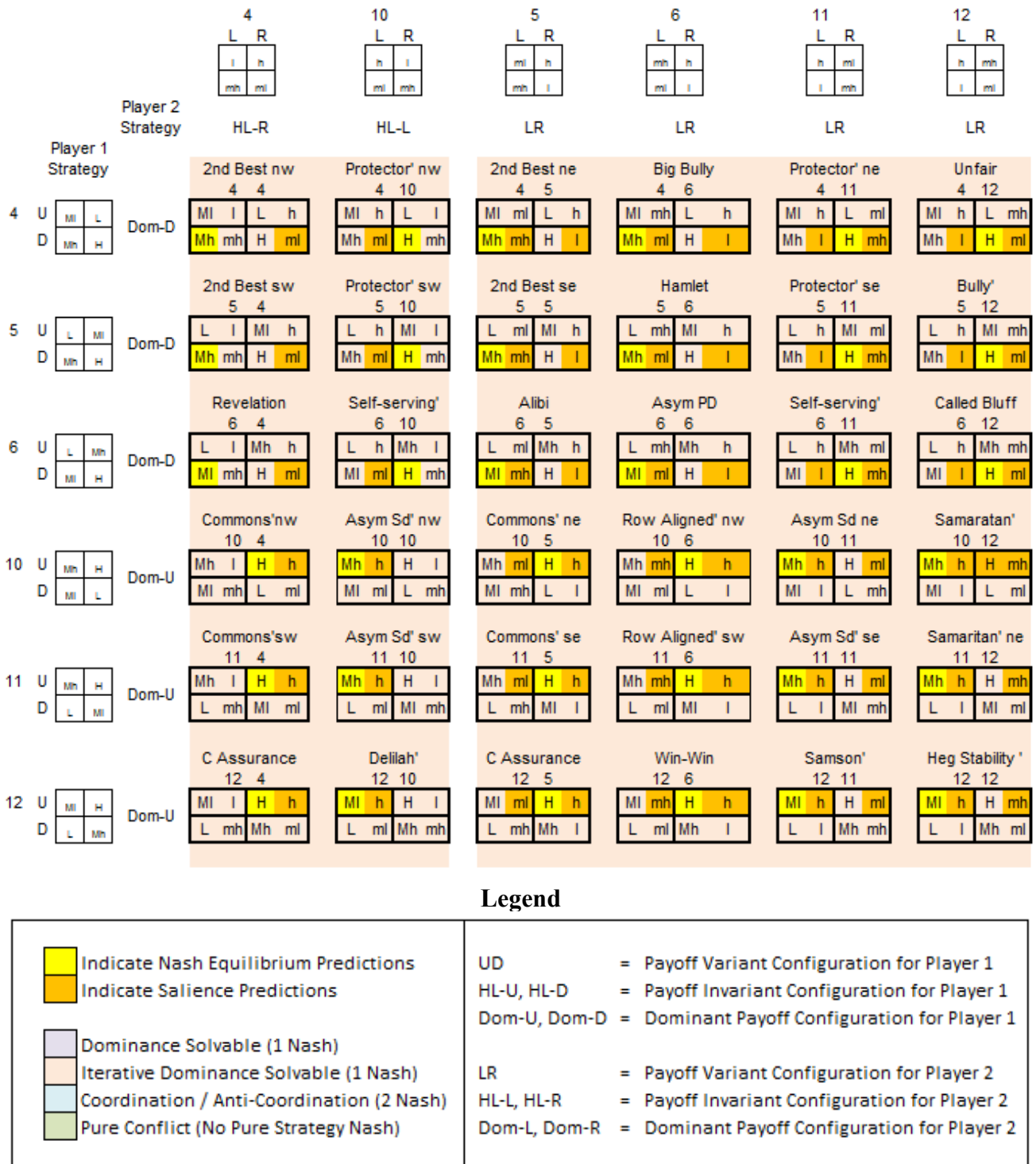
Figure 7. Strictly ordinal 2 × 2 dominance solvable games with dominant strategy for P1.
