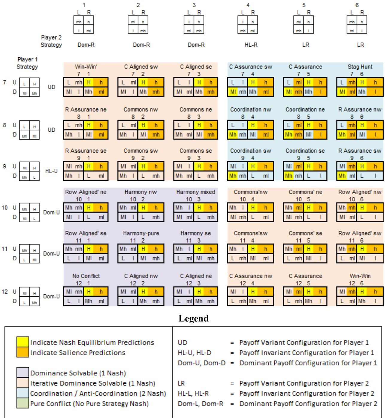
Figure 4. The class of 144 strictly ordinal 2 \times 2 games (games 7–1 through 12–6).
