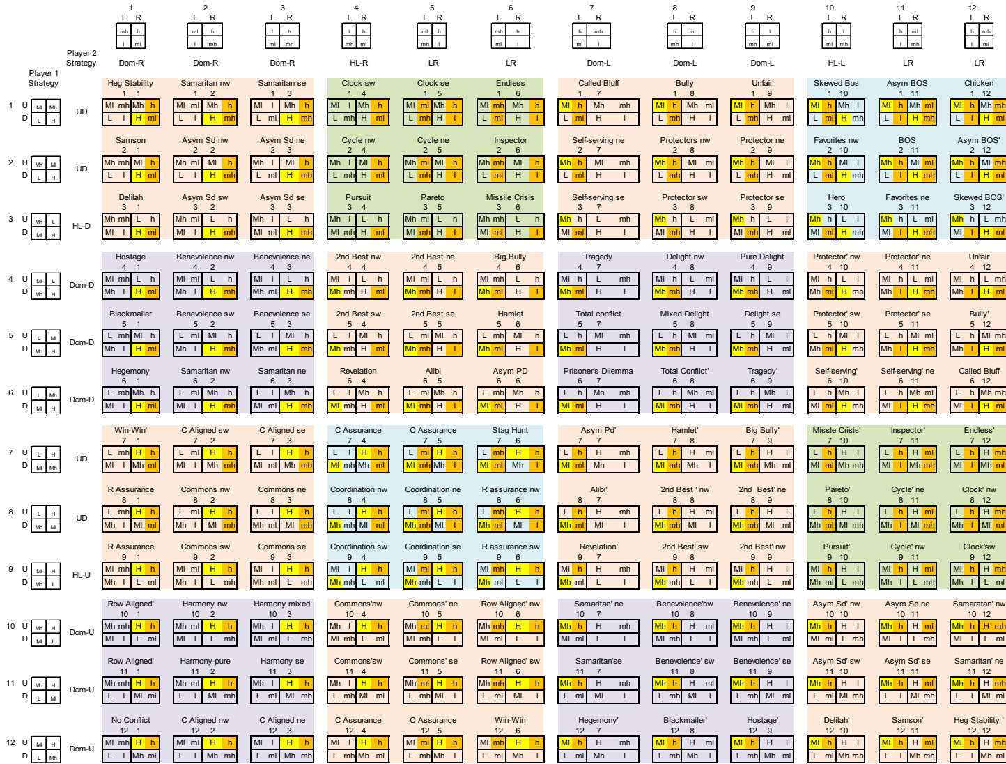
Figure A1. Robinson and Goforth's Taxonomy of 144 Strictly Ordinal Games (Composite of Figures 2–5).
