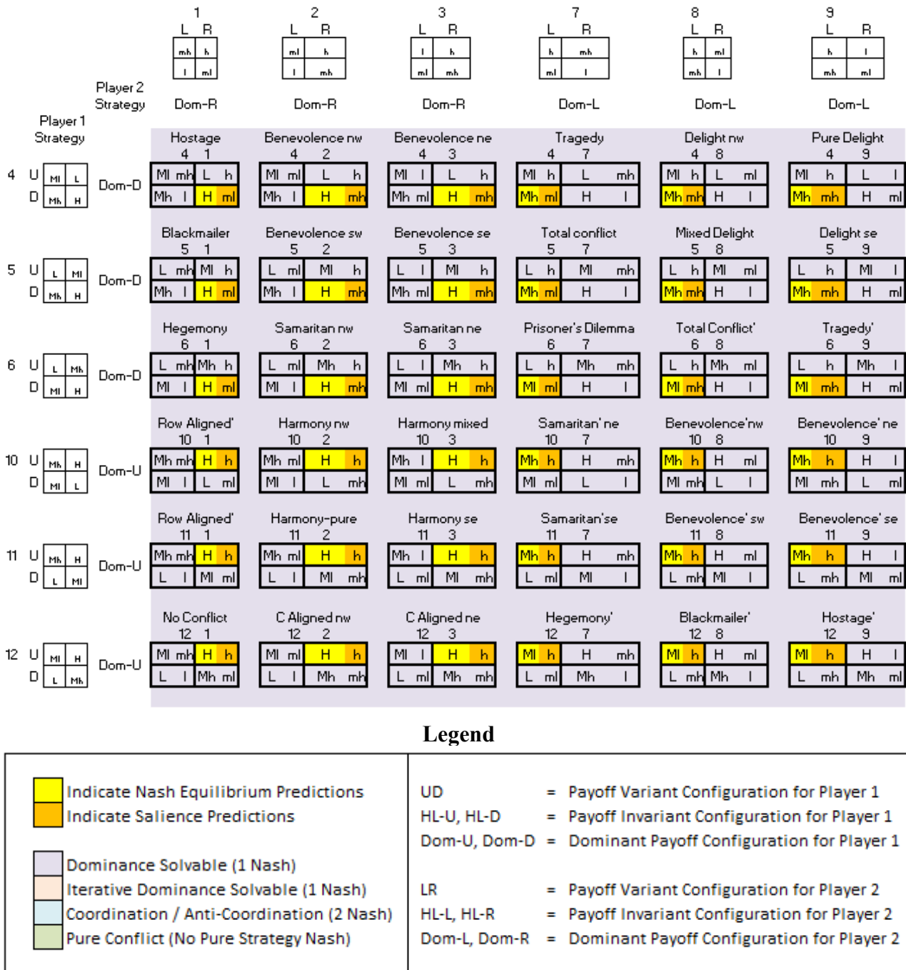
Figure 6. Strictly ordinal 2 \times 2 games containing a dominant strategy equilibrium.
