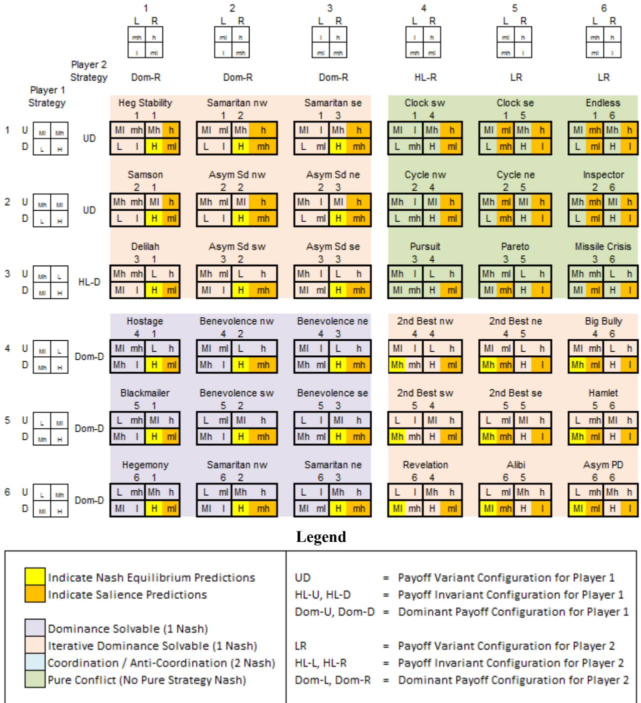
Figure 2. The class of 144 strictly ordinal 2 × 2 games (games 1–1 through 6–6).
