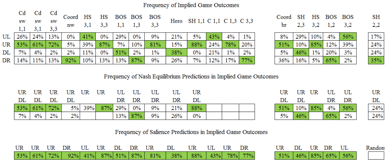
Figure 21. Observed Frequency of Implied Game Outcomes across all 20 Games.
