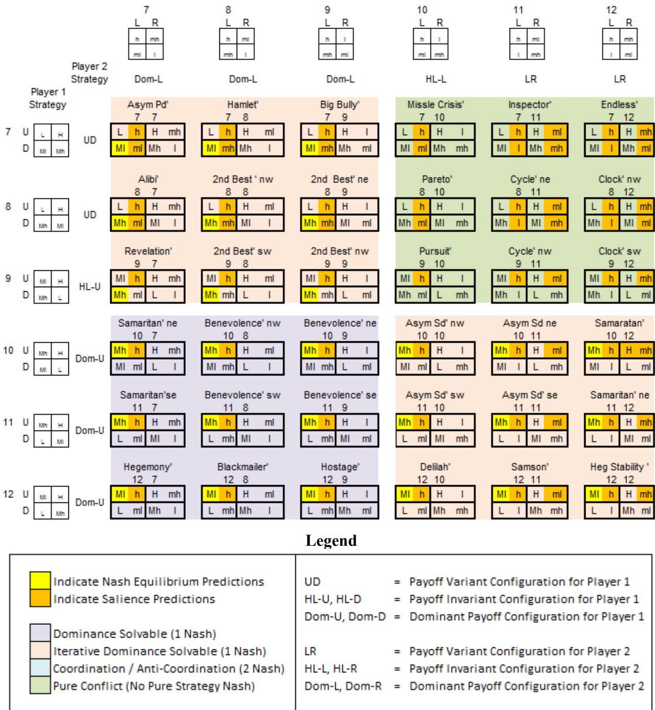
Figure 5. The class of 144 strictly ordinal 2 \times 2 games (games 7–7 through 12–12).
