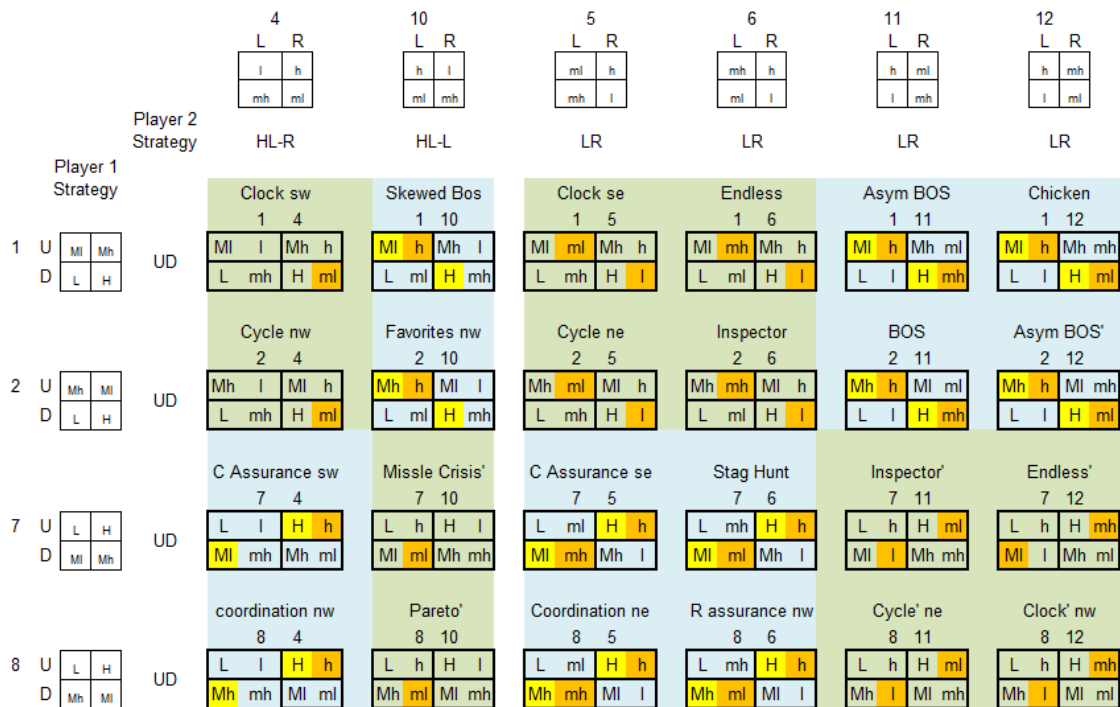
Figure 11. Implications of “other-payoff salience” in Cycle and Coordination Games for Player 1.
