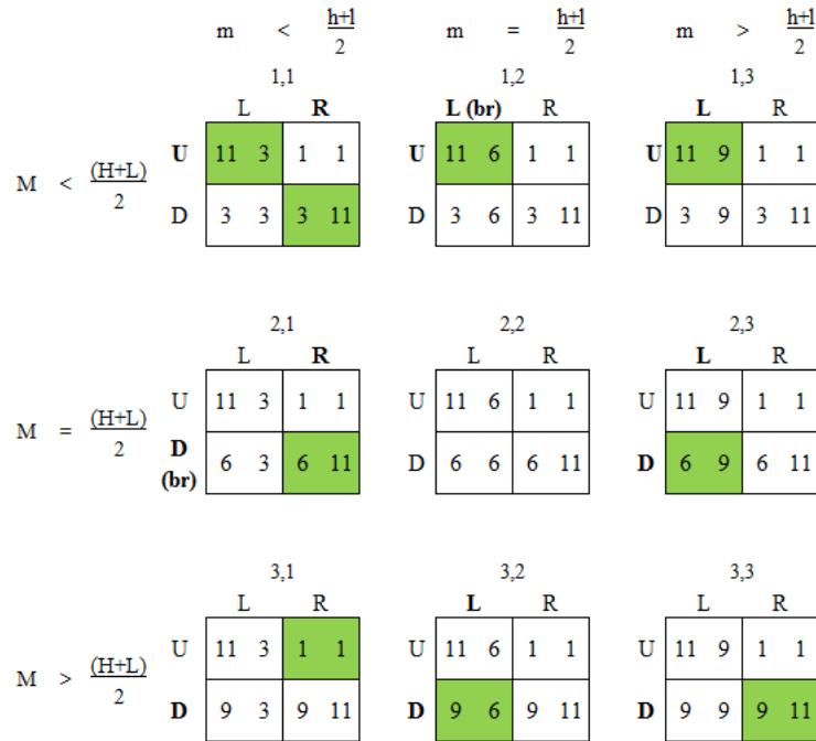
Figure 13. Testing Sensitivity of Play in a Payoff Variable Game.
