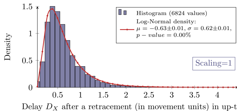
Figure 6. Measured and log-normal fit density of the delay in an up-trend with scaling one for S&P100 stocks. The data are visualized with a histogram from zero to five with a bin size of 0.11.
