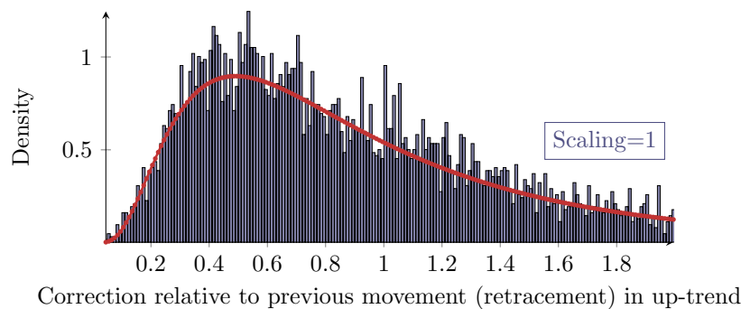
Figure 7. More detailed (finer) histogram of Figure 4 with scaling one from zero to two with a bin size of 0.01.
