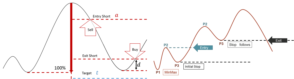
(a) Parameters a and t with exemplary realizations of the retracement X and delay d . (b) Entry at trend beginning and the following stop at the last low.
