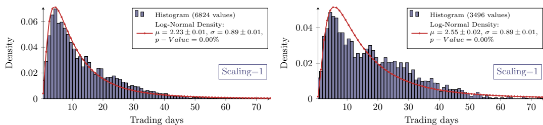
(a) Retracement duration Y in up-trend ( Mean = 13.0 ) (b) Retracement duration Y in down-trend ( Mean = 17.6 )
