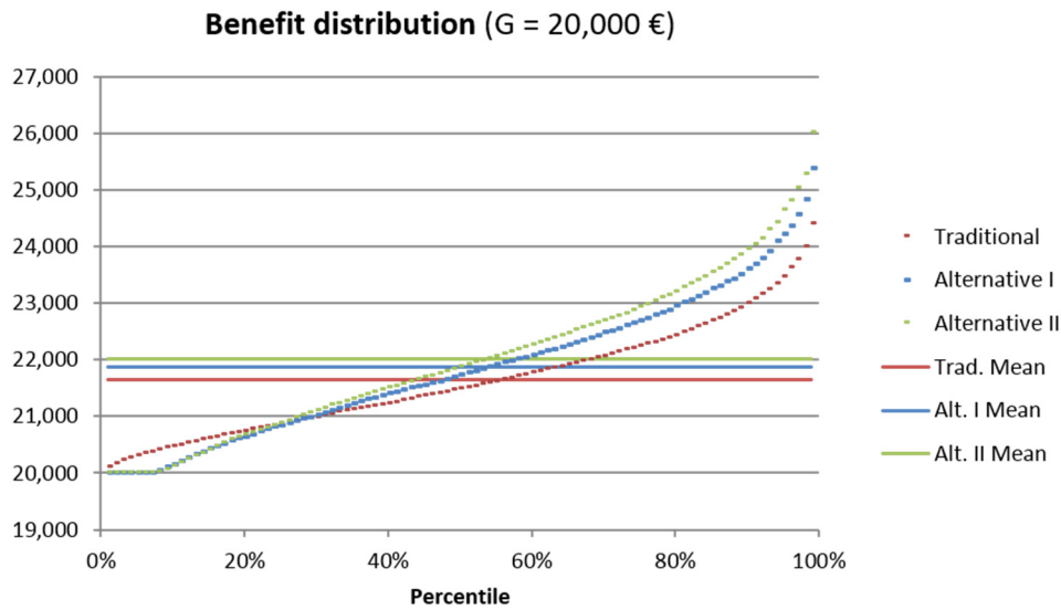
Figure 5. Benefit distribution of products with the same PVFP and reduced SCR_{mkt} , based on the traditional product with q = 5\% .
