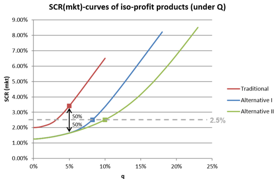
Figure 4. Comparison of products with the same PVFP and reduced SCR_{mkt} , based on the traditional product with q = 5\% .
