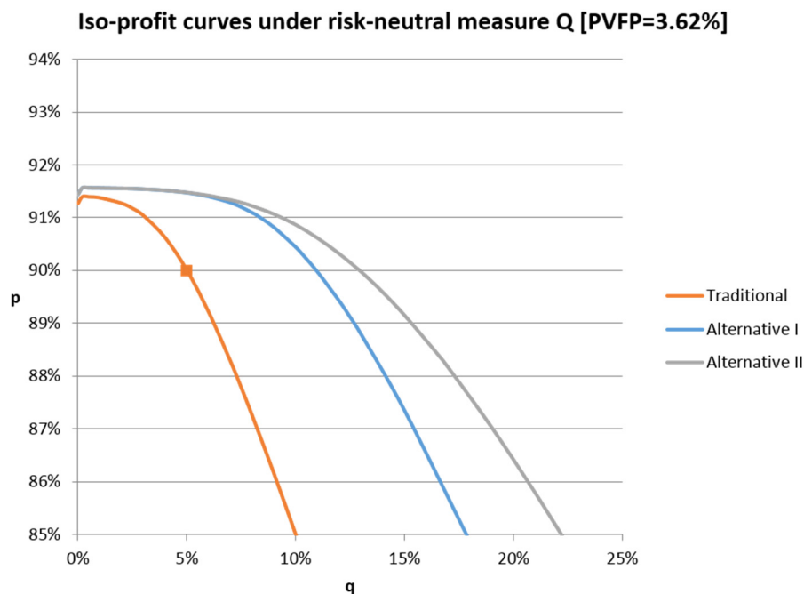
Figure 1. Iso-profit curves with PVFP = 3.62\% (based on the traditional product with p = 90\% and q = 5\% ).
