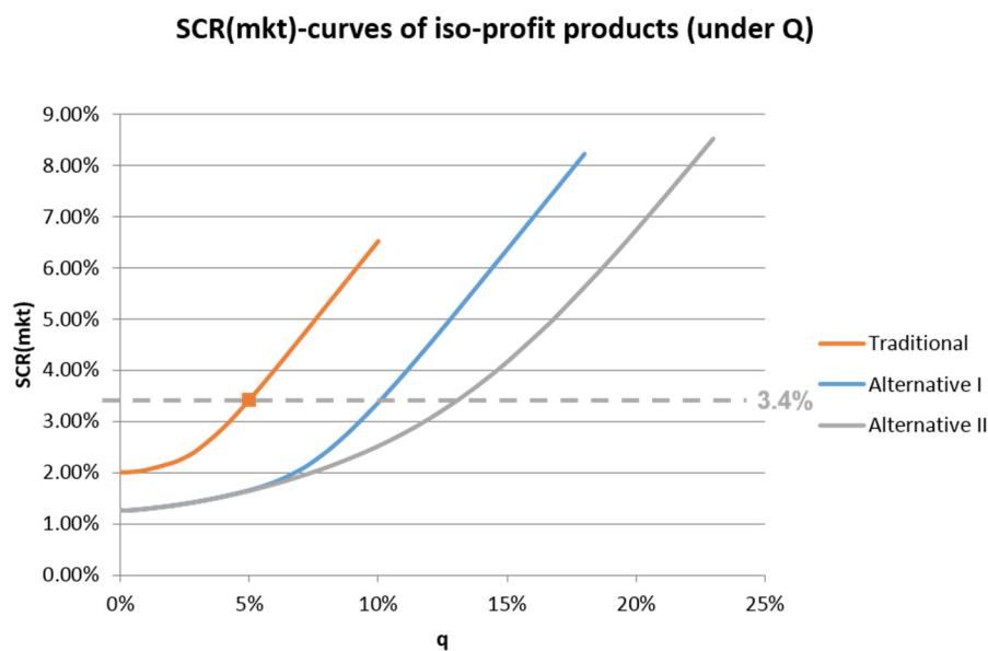
Figure 2. SCR_{mkt} curves of the iso-profit products.
