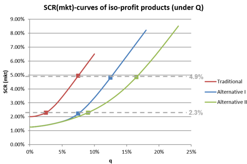
Figure 6. Comparison of products with the same PVFP and the same SCR_{mkt} , based on traditional products with q = 2.5\% ( SCR_{mkt} = 2.3\% ) and q = 7.5\% ( SCR_{mkt} = 4.9\% ).
