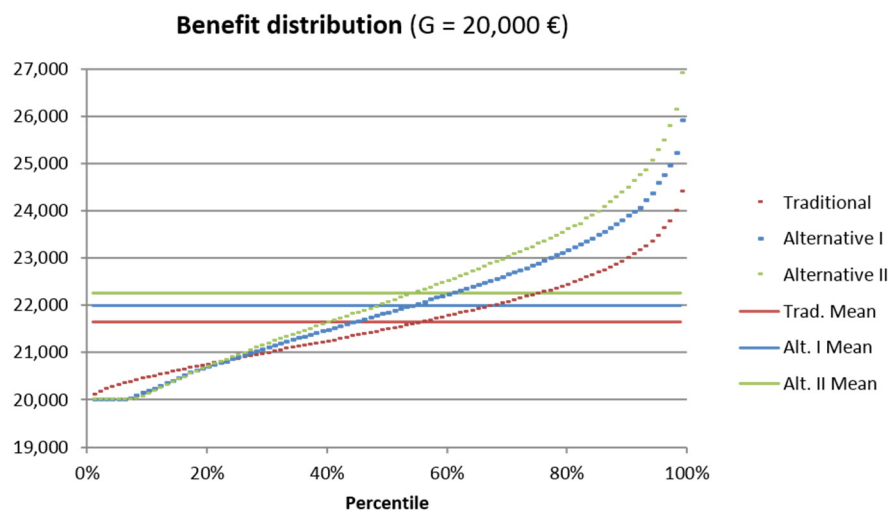
Figure 3. Benefit distribution of products with the same PVFP and the same SCR_{mkt} , based on the traditional product with q = 5\% .
