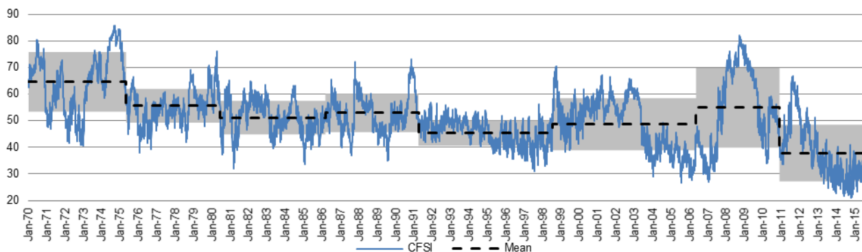
Figure 7. Daily CFSI compared to the mean and standard deviation (shaded region) of stress in each sub-period.
