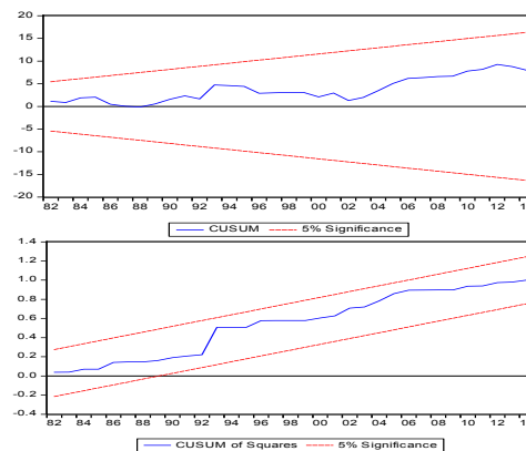
Figure A1. CUSUM and CUSUMQ results for Model 1: PI = f(PUINV, OPEN, Y, RER, R, PSC) .
