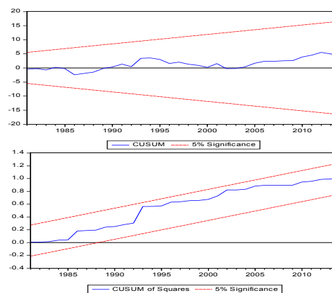
Figure A2. CUSUM and CUSUMQ results for Model 2: PI = f(PUINV, OPEN, Y, RER, R) .
