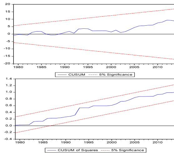
Figure A3. CUSUM and CUSUMQ results for Model 3: PI = f(PUINV, OPEN, Y, RER R, DMG) .
