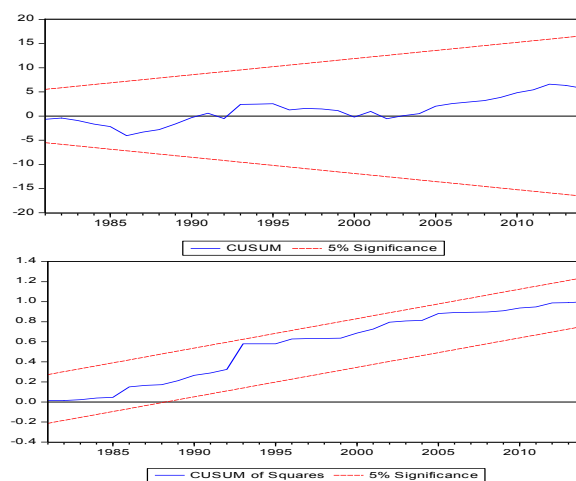
Figure A5. CUSUM and CUSUMQ results for Model 5: PI = f(PUINV, OPEN, Y, RER R, FDP) .
