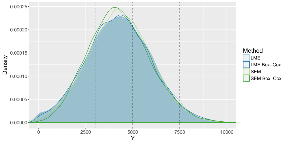
Figure 13: Normal scenario 2, predicted and true density
