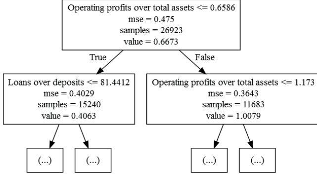
Figure 2: Example of a Decision Tree Estimation
