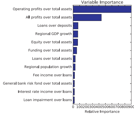
Figure 4: The Importance of the Included Variables for the Estimation
