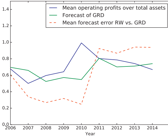
Figure 3: Mean Absolute Error per Year of Different Forecasting Techniques
