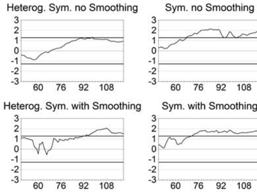
Figure 9: DM Statistics across Different Window Sizes of Equations (5) and (10) for the Swedish Kronor-US Dollar Exchange Rate
