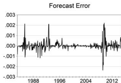
Figure 2: Forecast Comparison between Equation (5) and (10) for the Pound-US Dollar Exchange Rate
