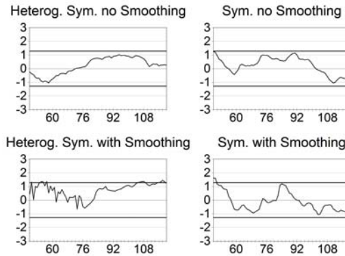
Figure 10: DM Statistics across Different Window Sizes of Equations (5) and (10) for the Swiss Franc-US Dollar Exchange Rate
