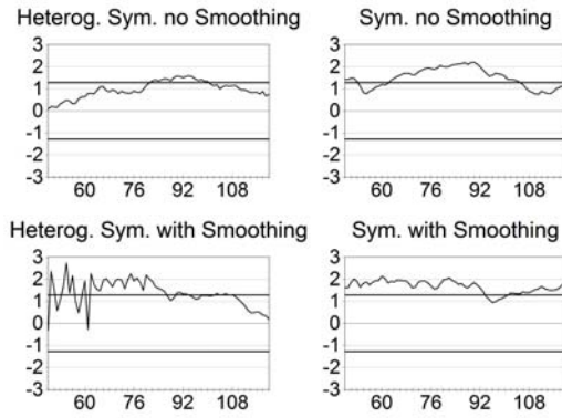
Figure 8: DM Statistics across Different Window Sizes of Equations (5) and (10) for the Danish Kroner-US Dollar Exchange Rate
