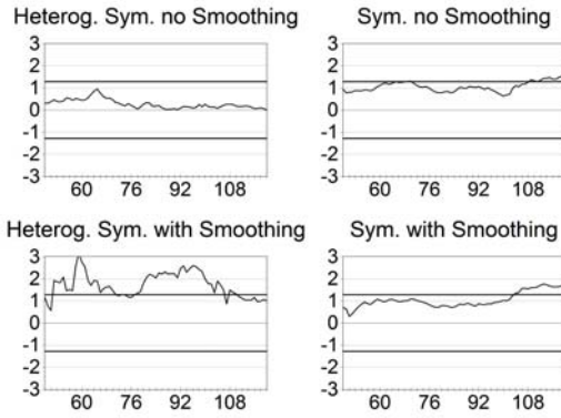
Figure 7: DM Statistics across Different Window Sizes of Equations (5) and (10) for the Australian Dollar-US Dollar Exchange Rate
