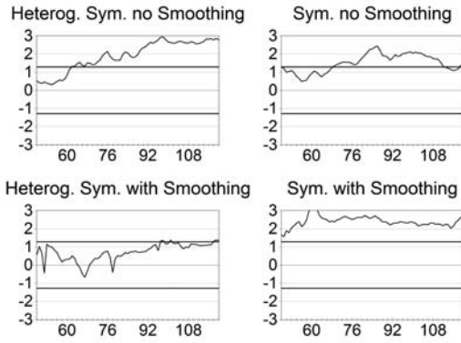
Figure 5: DM Statistics across Different Window Sizes of Equations (5) and (10) for the Pound-US Dollar Exchange Rate
