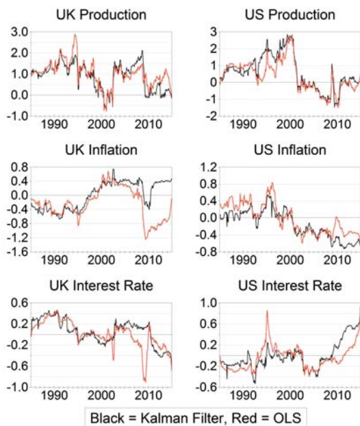
Figure 1: Estimated Coefficients of a Kalman Filter Model and OLS
