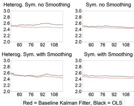
Figure 4: MSPE across Different Window Sizes of Equations (5) and (10) for the Pound-US Dollar Exchange Rate
