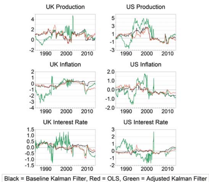
Figure 3: Coefficients Estimated with Different Kalman Filter Models or OLS
