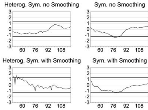
Figure 6: DM Statistics across Different Window Sizes of Equations (5) and (10) for the Canadian Dollar-US Dollar Exchange Rate
