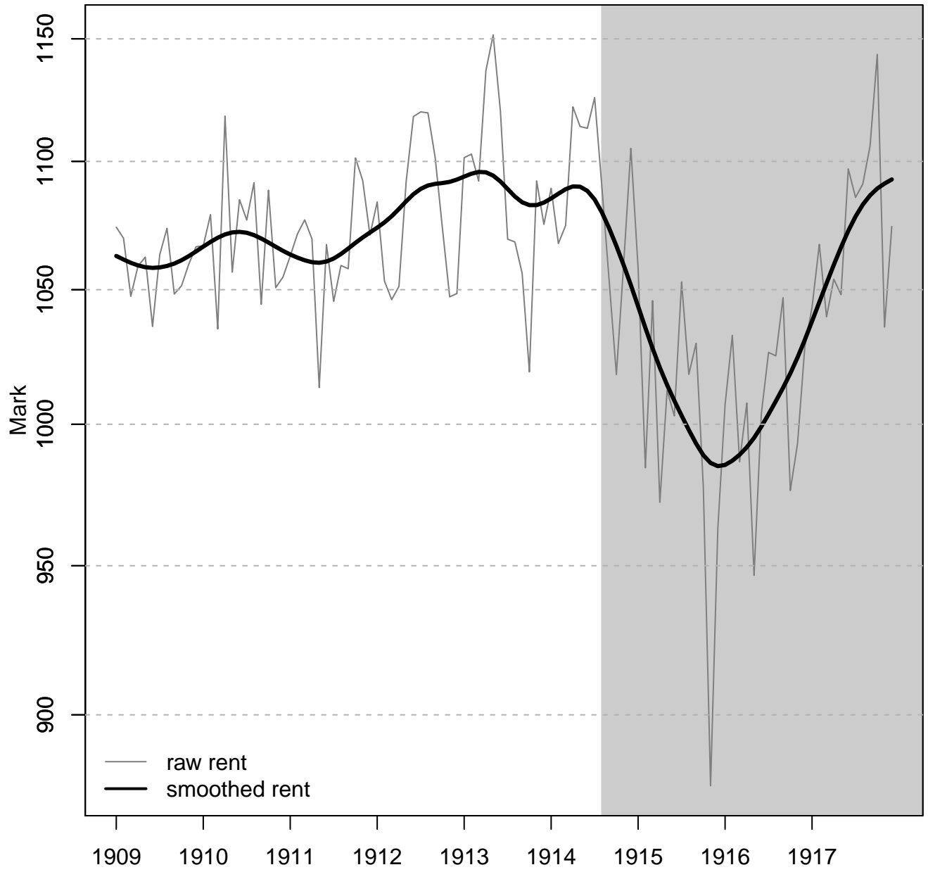
Figure 6: Quality-adjusted housing rent in Berlin, 1909–1917
