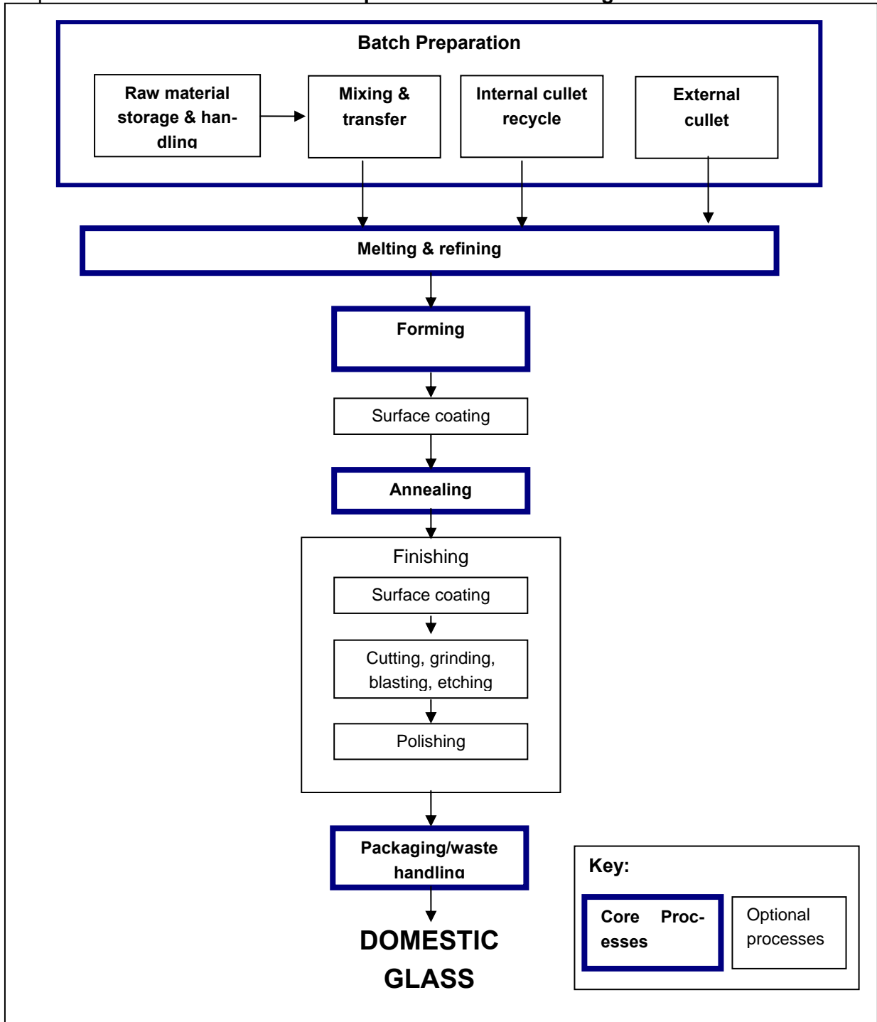
Graph 28: Processes involved in the production of domestic glass
