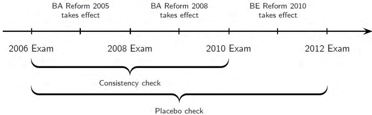
Figure 4.2. Robustness Checks.
