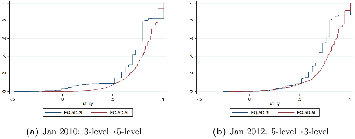
Figure 6: Cross-mapping based on independent domain-specific bivariate models
