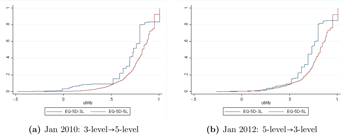
Figure 7: Cross-mapping based on the joint model with between-domain correlation
