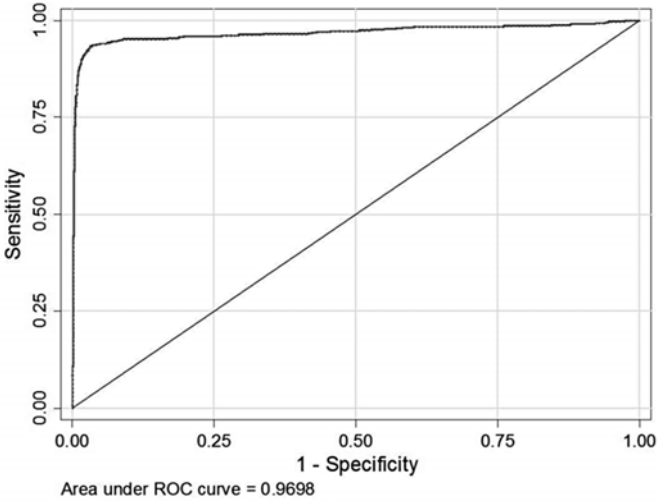
Figure 4: ROC curves
