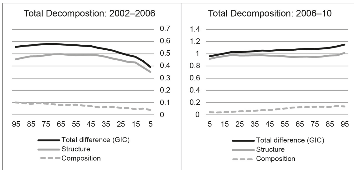
Figure 8: Decomposition Analysis
