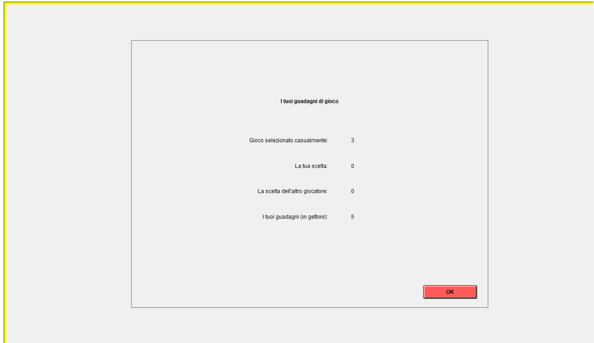
SCREENSHOT 7B
