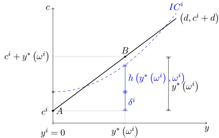
Figure 3: Labor supply distortions, Example 2.
