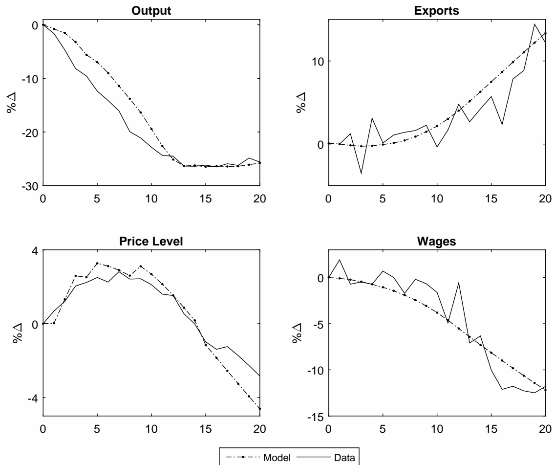
Figure 12: Model Performance
