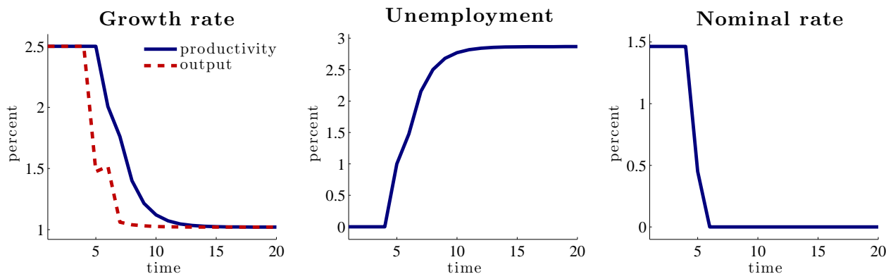
Figure 4: An example of transition toward the unemployment steady state.
