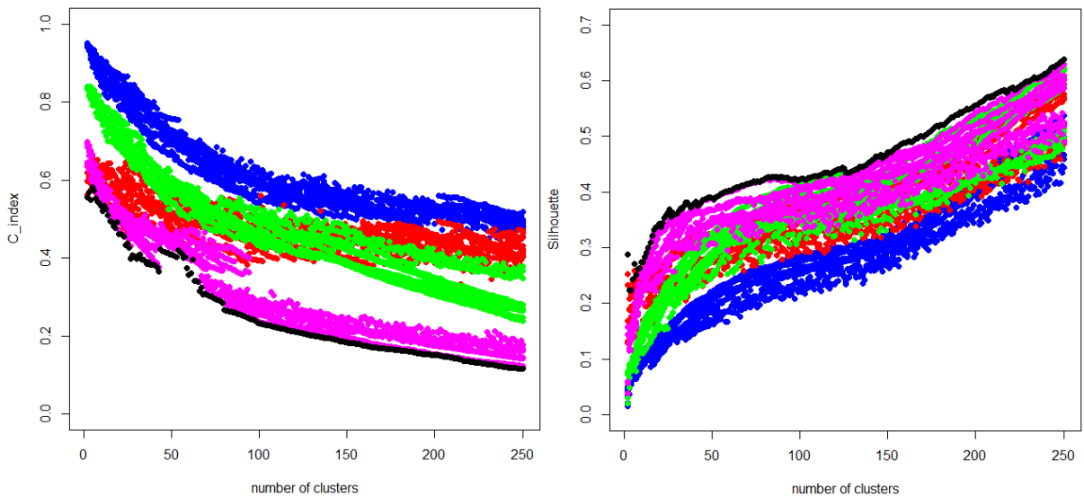
Figure 7: Smart-Vali-plots of YAML-500 for C-Index (left: to be minimized) and Silhouette index (right: to be maximized) from the package NbClust ; Standard TM colors: BWSM , GVSM(TT) , LSA , LSA25
