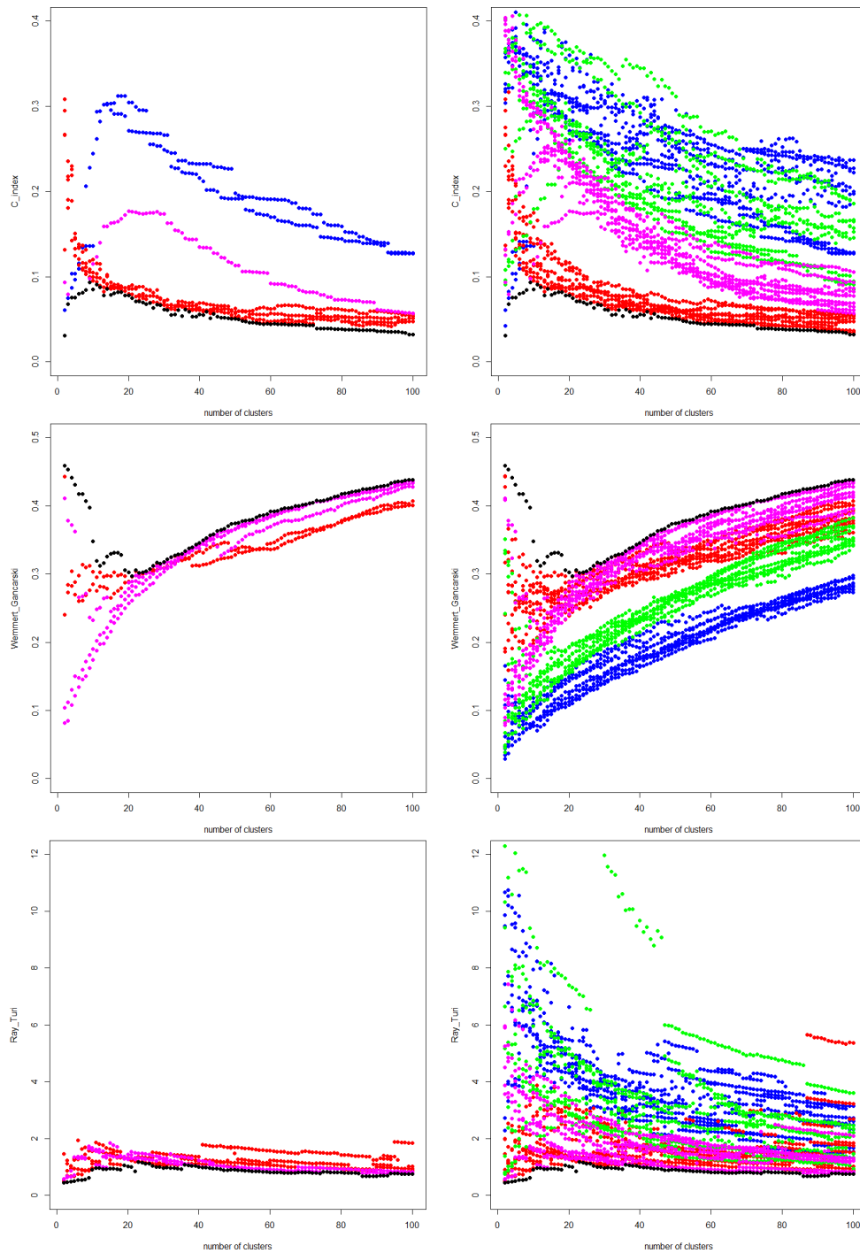
Figure 8: Smart-Vali-plots of YAML-1140 for the indices: C-Index, Wemmert-Gancarski, Ray-Turi from the clusterCrit package; Standard TM colors: BVSM , GVSM(TT) , LSA , LSA25
