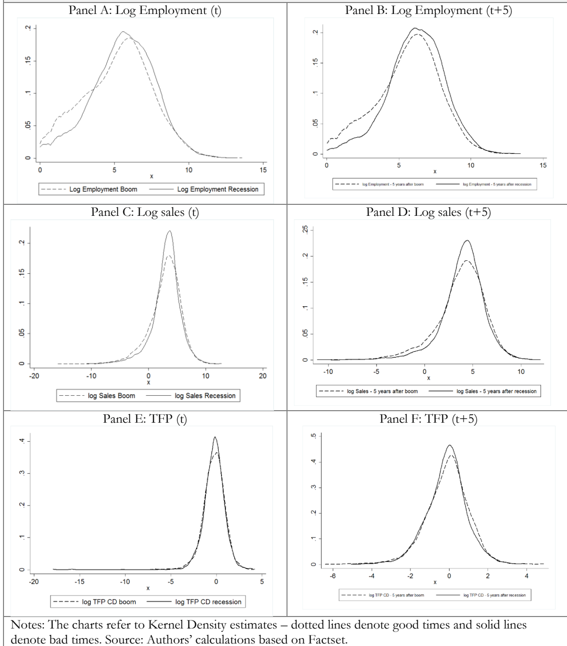
Figure 5: Selection effect of recessions: Contemporaneous (left) and 5-year (right)
