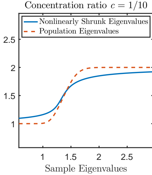
Figure 7: Nonlinearly shrunk eigenvalues as a function of sample eigenvalues. The population eigenvalues come from the Beta(0.1, 0.1) distribution, shifted so the support is [1, 2] . The optimal shrinkage transformation is highly nonlinear. The population eigenvalues are also plotted for reference as the dashed line. They are not the same as the shrunk eigenvalues, and are more spread out.
