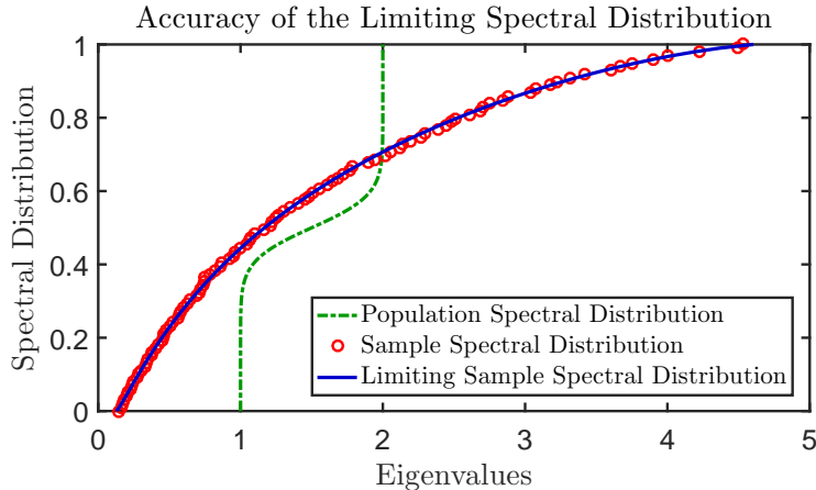
Figure 5: Three spectral distributions for N = 100 and T = 200 . The population spectral distribution is the Beta(0.1,0.1) distribution shifted so the support is [1, 2] . Circles show the sample spectral distribution from one Monte Carlo simulation. One can observe that the sample eigenvalues are nowhere near their population counterparts, but their location is well predicted by the limiting spectral distribution F that comes out of equation (9.15).
