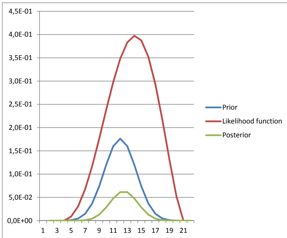
Fig. 1. Prior distribution, posterior distribution and likelihood for q
