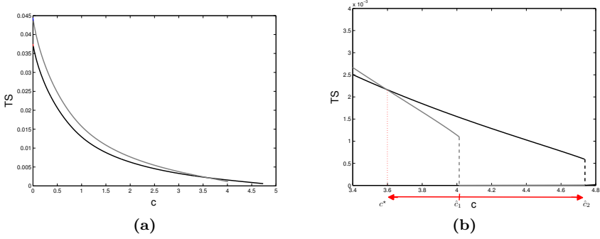
Fig. 9 Total surplus when the indifference point is in the region with zero production. Parameters: (\beta, \rho, \phi) = (1, 10, 50) . Grey curves correspond to partial collusion, whereas the black ones correspond to full collusion. c^* \approx 3.6 , \hat{c}_1 \approx 4.01 , \hat{c}_2 \approx 4.74 . For all c_0 \in (c^*, \hat{c}_2) , total surplus is higher if firms collude in the product market
