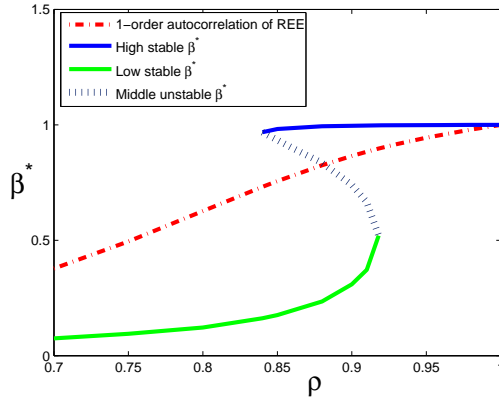
Figure 9: First-order autocorrelation coefficient of REE inflation (dotted red curve), stable BLE \beta^* with respect to \rho (bold curves), unstable BLE \beta^* (dotted curve), where \gamma = 0.075, \sigma_u = 0.003162, \sigma_\varepsilon = 0.01, \delta = 0.99 .
