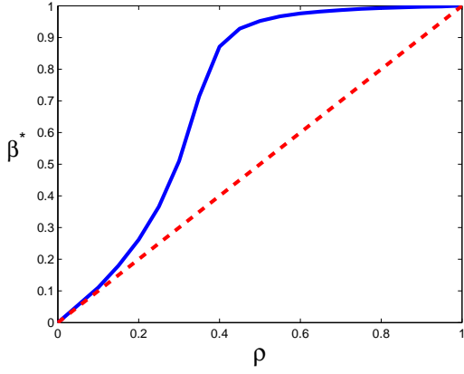
(a) first-order autocorrelation in BLE
