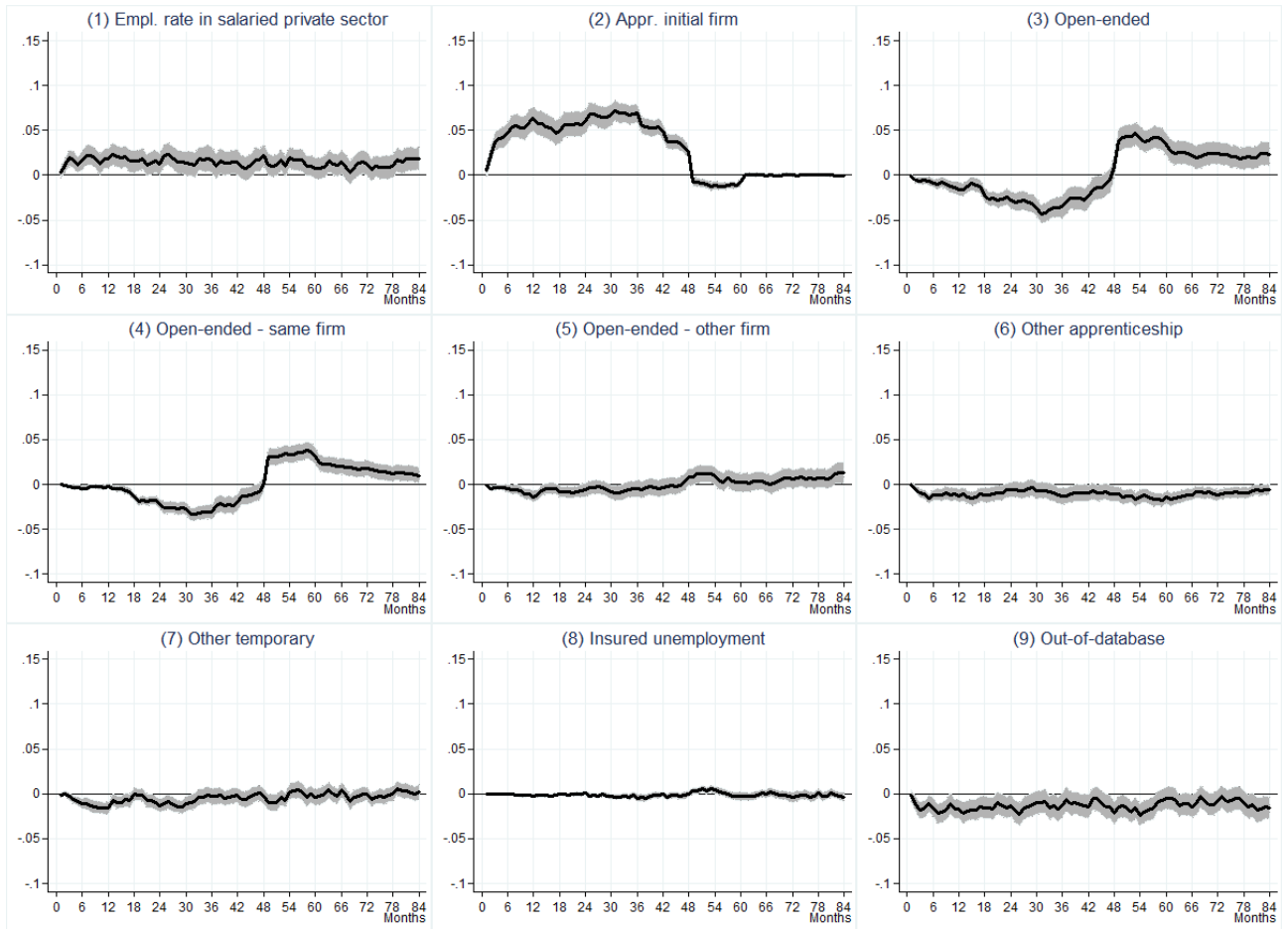
Figure 3: ATT on the Apprentices in the Next Seven Years
