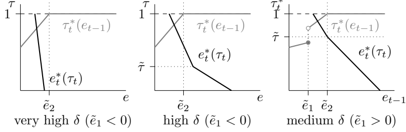
Figure C.1: Equilibrium Strategies
