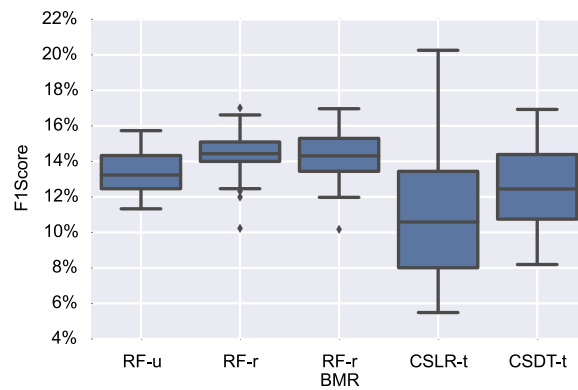
Fig. 9 Comparison of the random forest, logistic regression, Bayes minimum risk and cost-sensitive logistic regression algorithms. The best model selected by savings is not the same as the one selected by the F1 – Score
