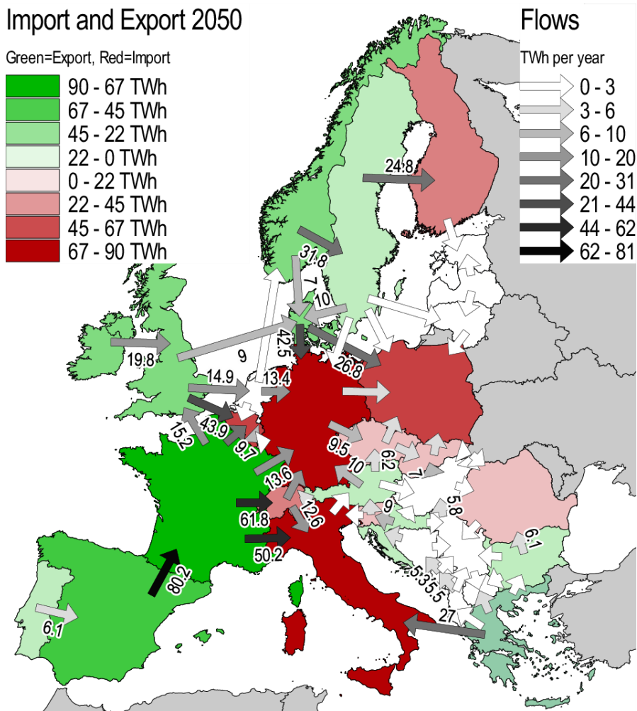
Figure 25: Import and export in TWh in the year 2050, calculated with NTC approach
