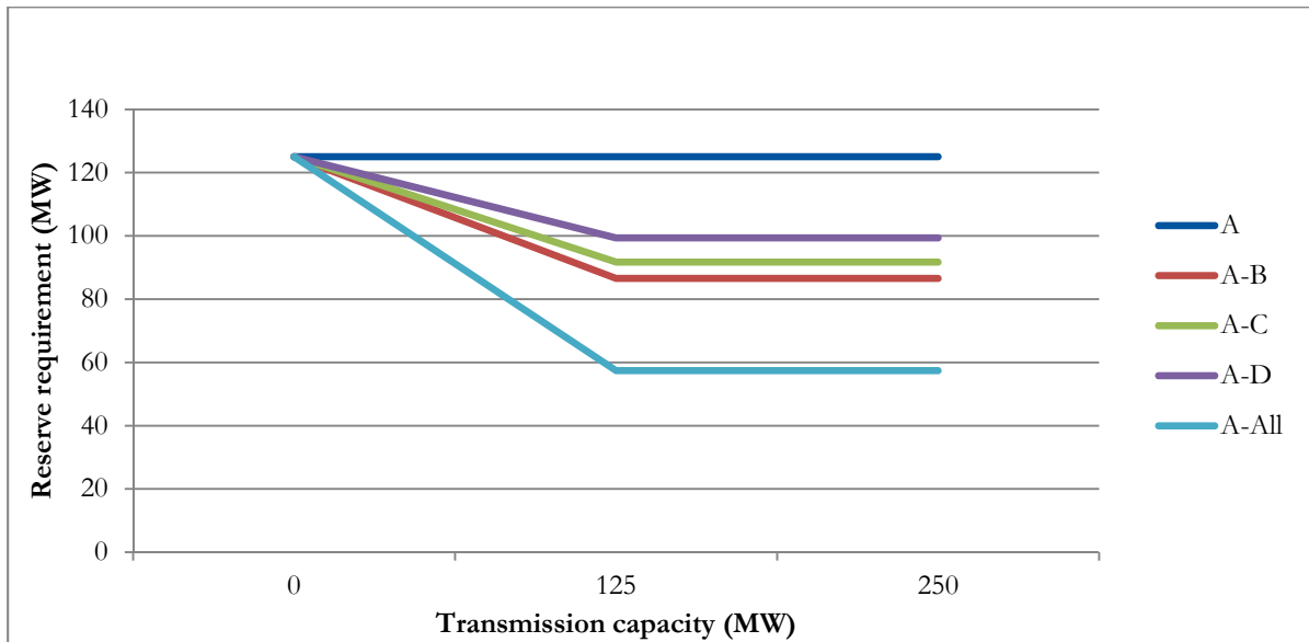
Figure B2: Operating reserve requirements for country A for different interconnection scenarios and levels of transmission capacity
