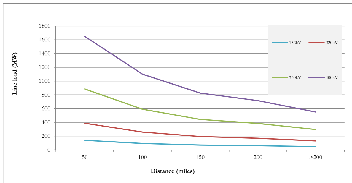
Figure A1: Piecewise power transfer function for candidate lines
