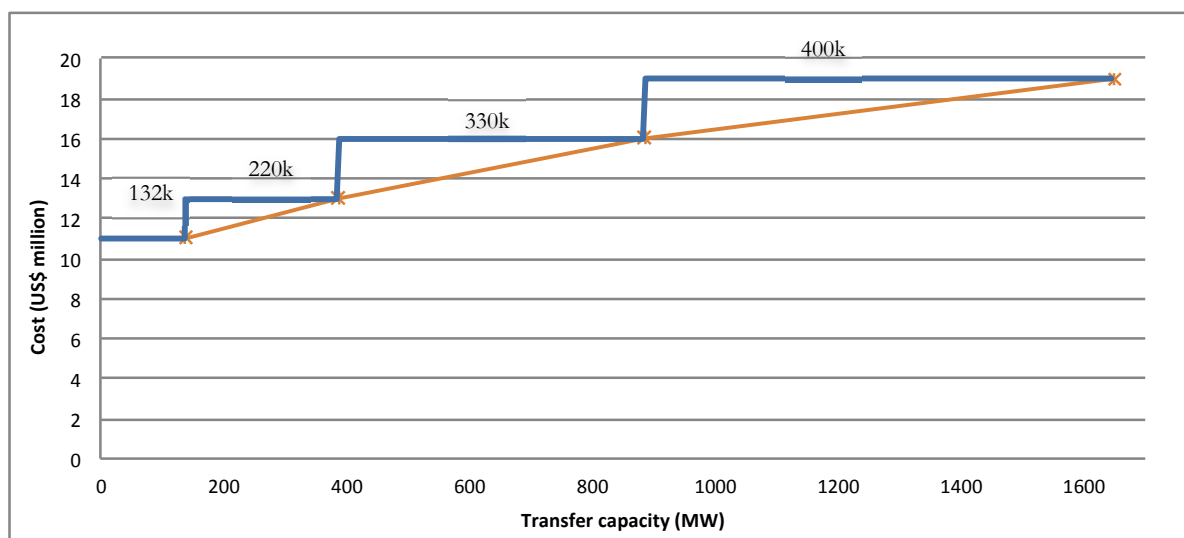
Figure A2: Relationship between cost and transfer capacity for the 0–50-mile range
