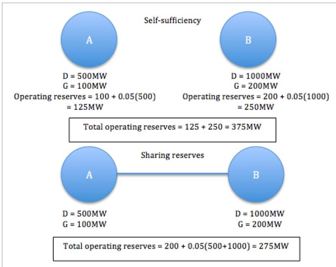
Figure B1: Benefits of sharing operating reserves
